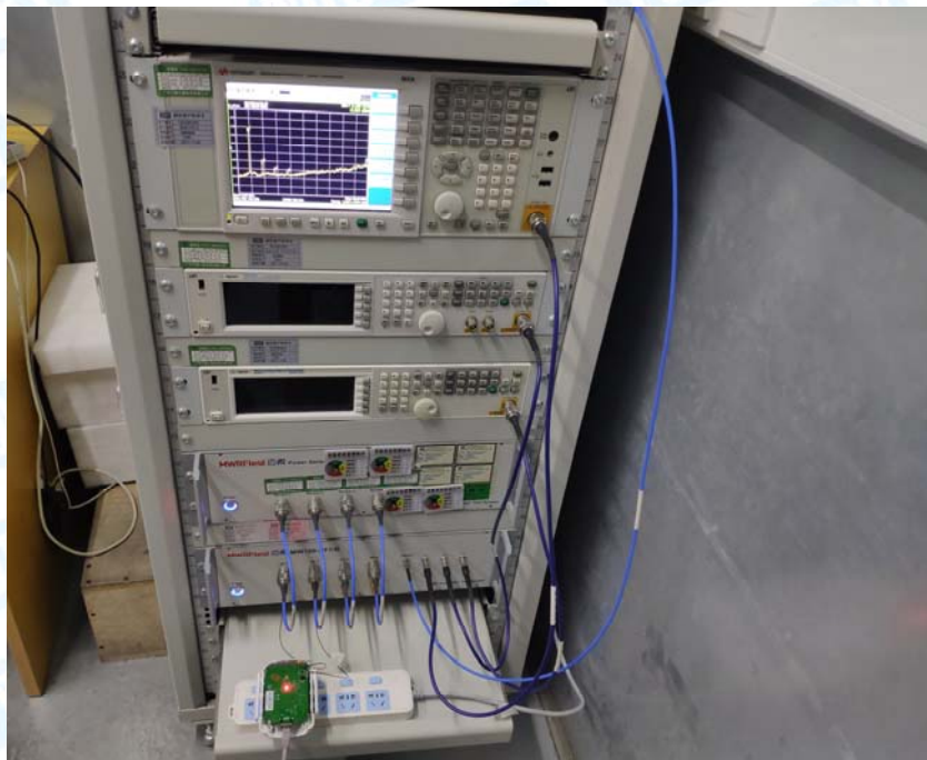
Photo of Setup for RF Conducted Test
