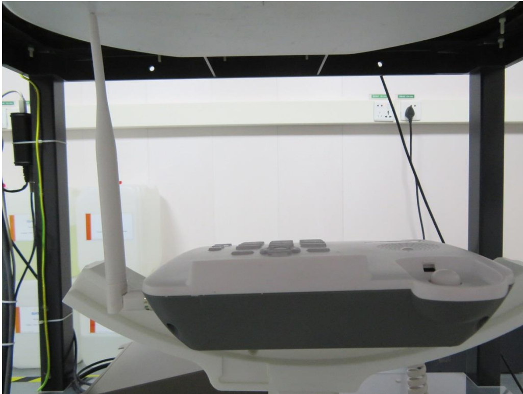
0mm body-worn Vertical-Bottom Side Setup Photo(90° )
