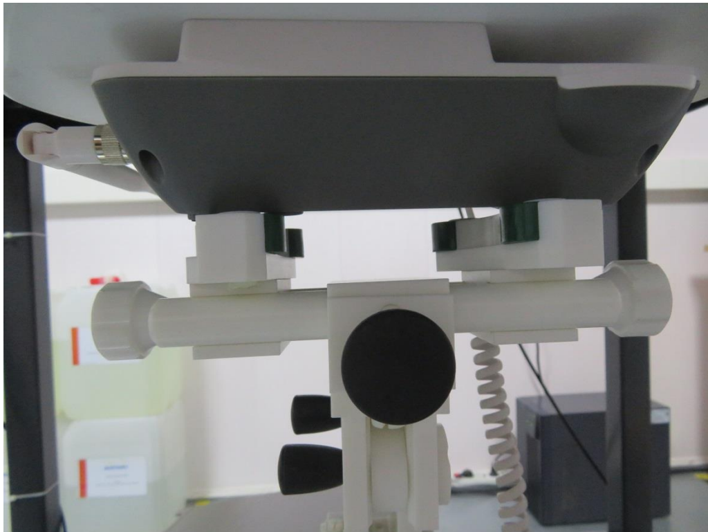
0mm body-worn Horizontal-Up Side Setup Photo(180° )
