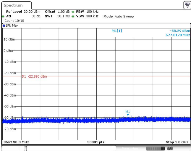
30MHz~1GHz
