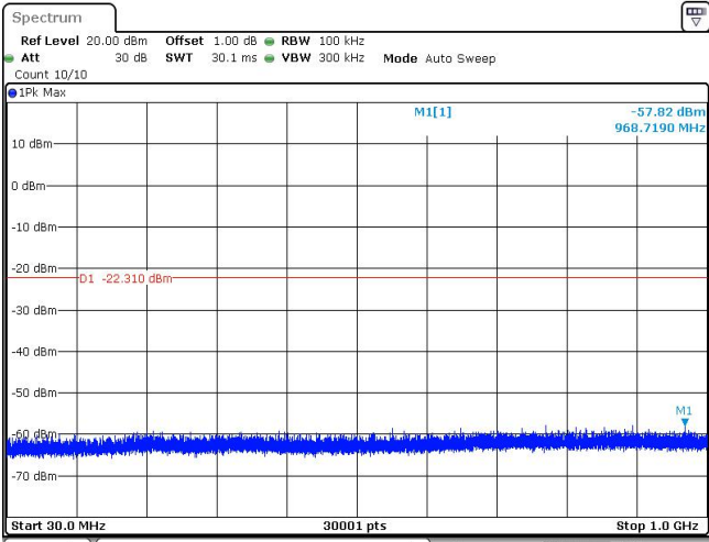
30MHz~1GHz
