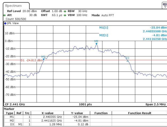
Middle channel
