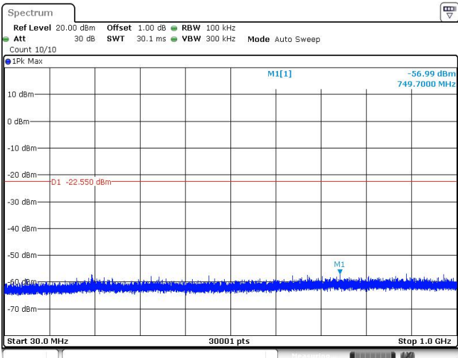
30MHz~1GHz
