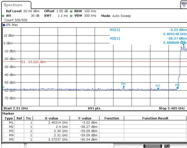
Hopping mode
