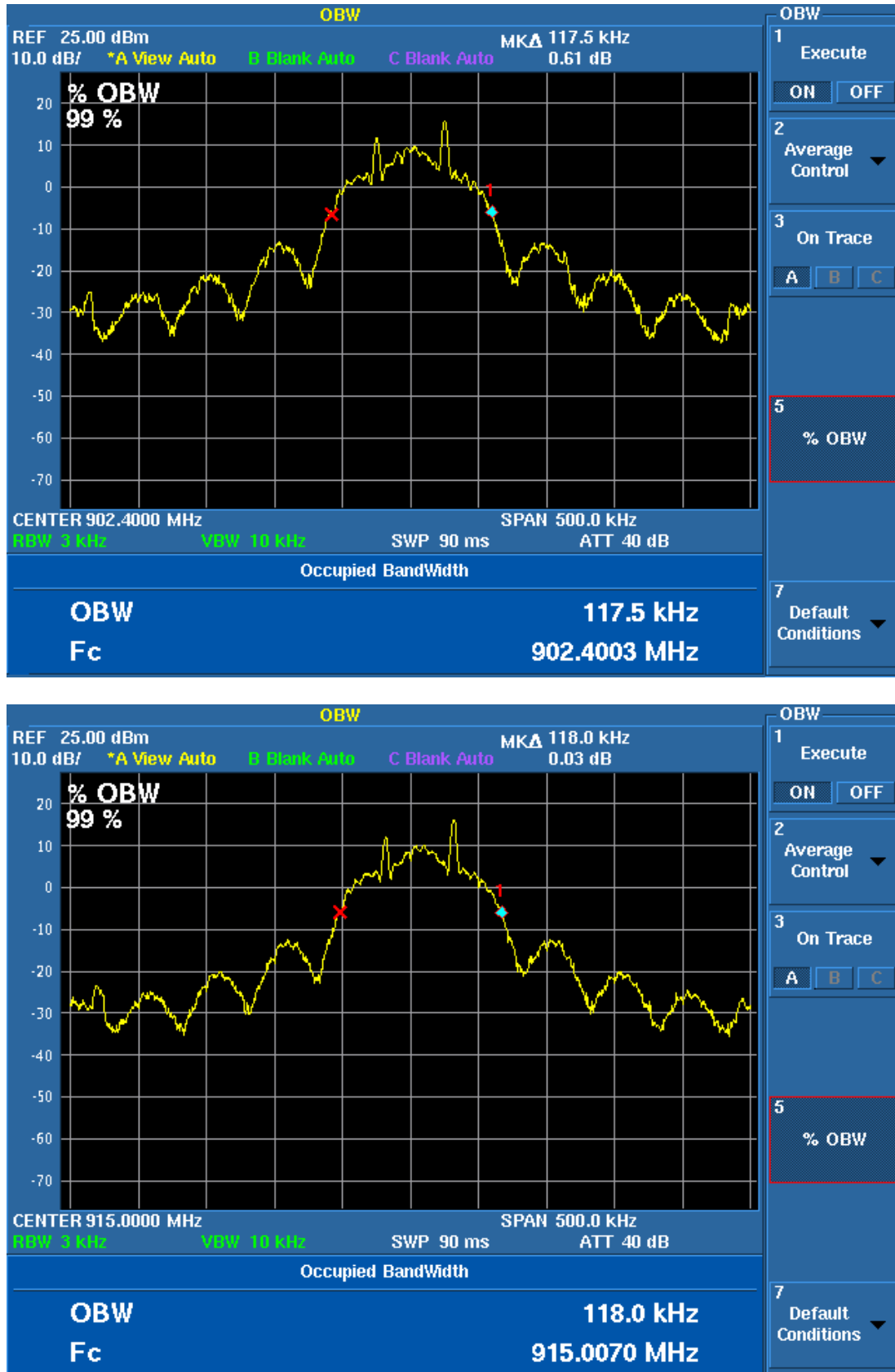
Figure 1. Occupied Bandwidth Plots
