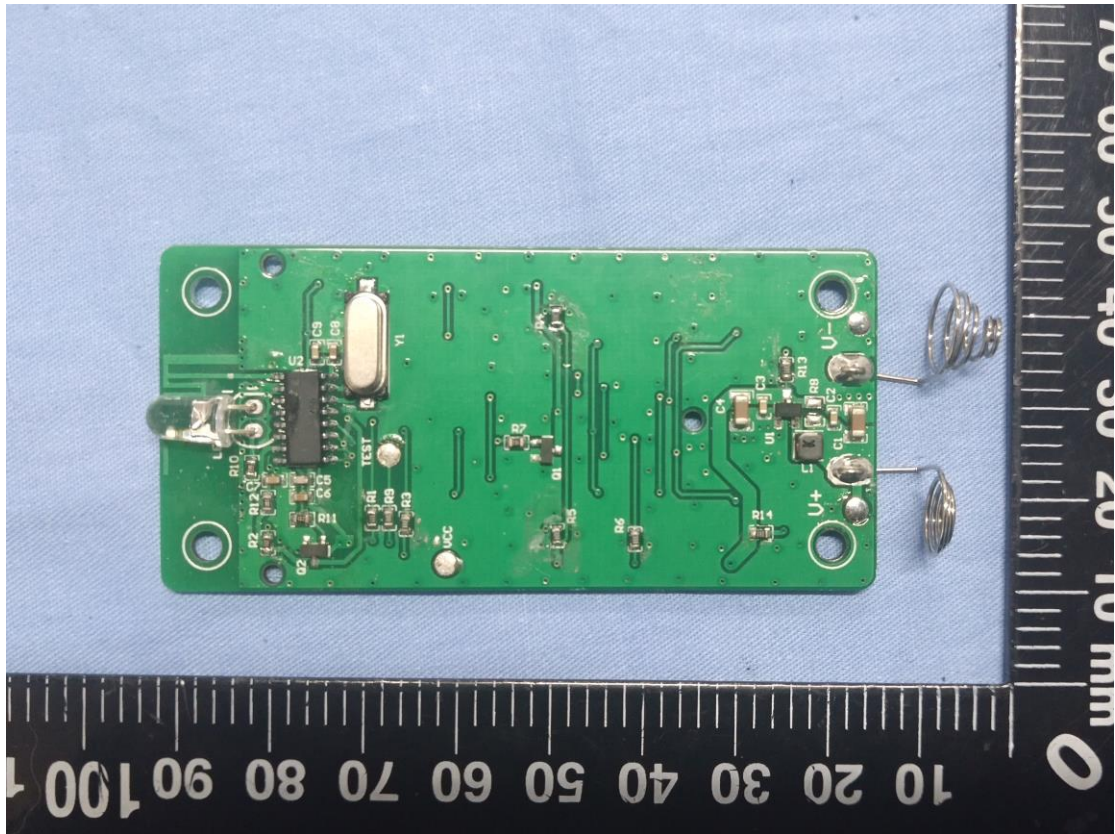
6. RF chip view
