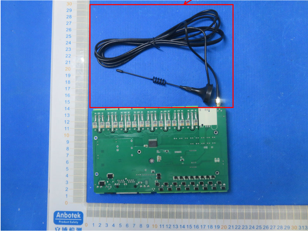
WIFI Antenna
