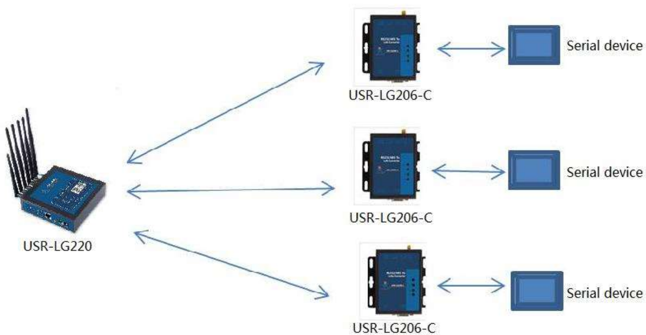
Figure 2 Application diagram
