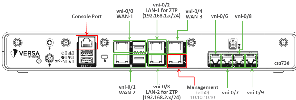
Figure 3: Port-to-VNI Mapping
