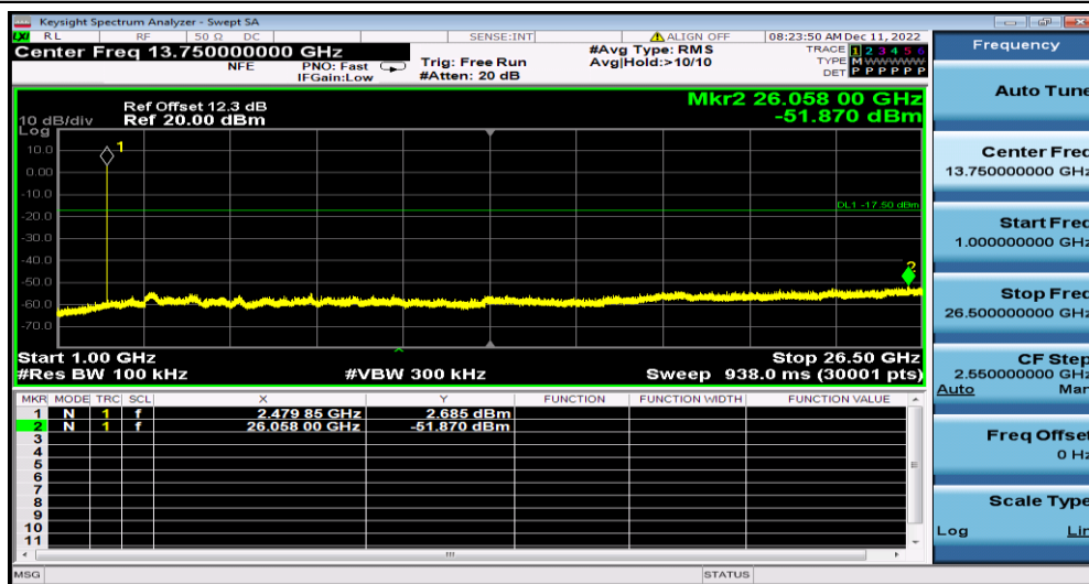
2DH5_Ant1_2480_1000~26500
