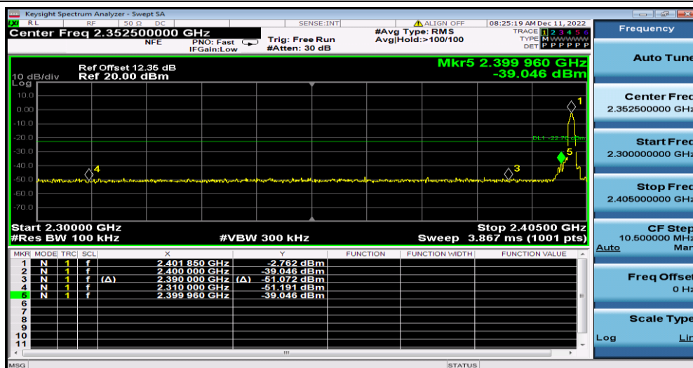
3DH5_Ant1_Low_2402
