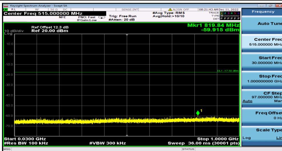
2DH5_Ant1_2480_30~1000
