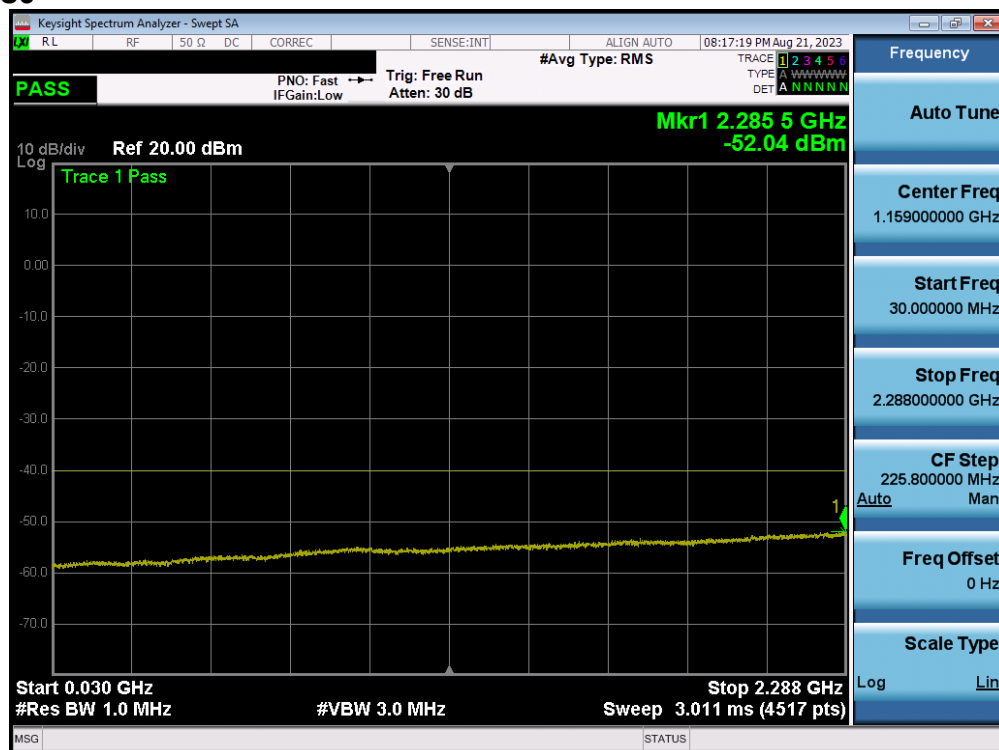
Plot 7-4. Conducted Spurious Plot (NR Band n30 - 5MHz QPSK - Low Channel)
