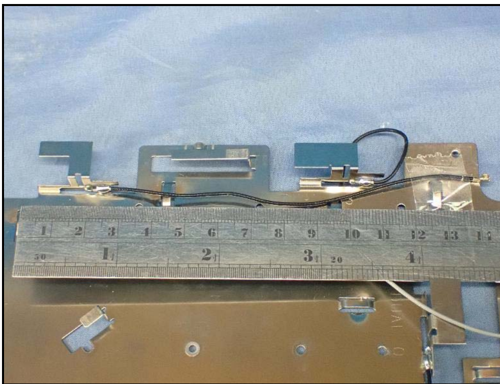
Antenna: SCANNING_baseline
