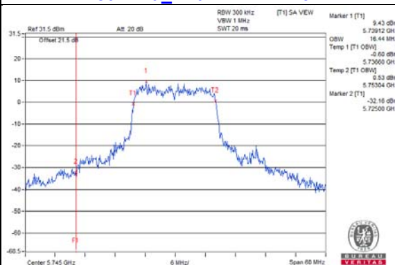
802.11a_Chain 7 / CH149
