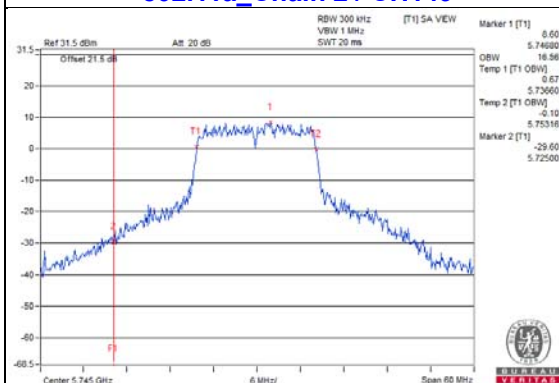
802.11a_Chain 4 / CH149
