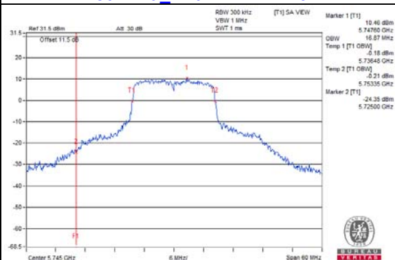
802.11a_Chain 3 / CH149
