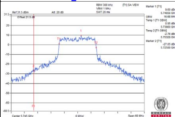
802.11a_Chain 7 / CH149
