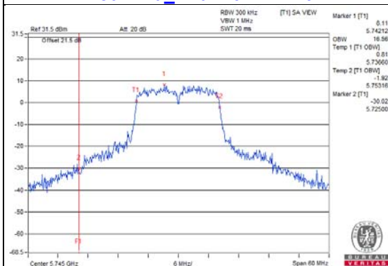
802.11a_Chain 6 / CH149
