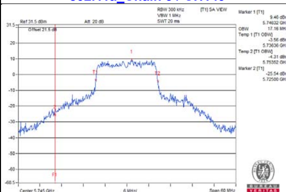
802.11a_Chain 5 / CH149
