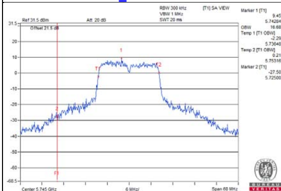
802.11a_Chain 6 / CH149
