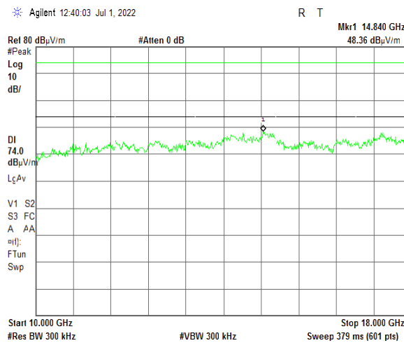
Plot 7.6.23 Radiated emission measurements from 10000 to 18000 MHz at the mid carrier frequency
