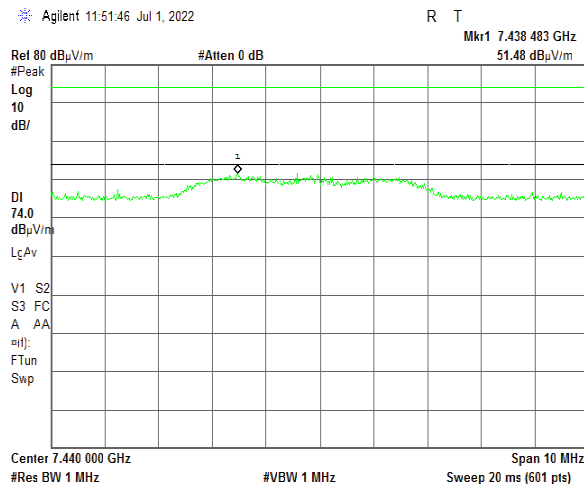
Plot 7.6.33 Radiated emission measurements at the fourth harmonic of low carrier frequency
