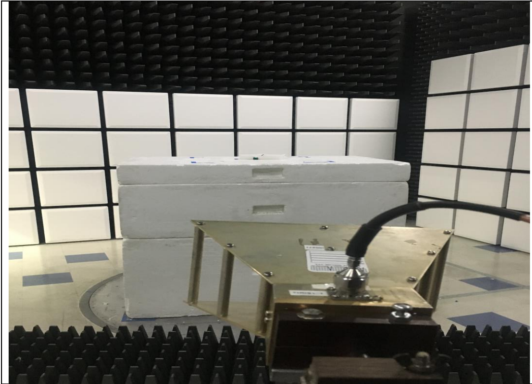
RF Radiated #2
