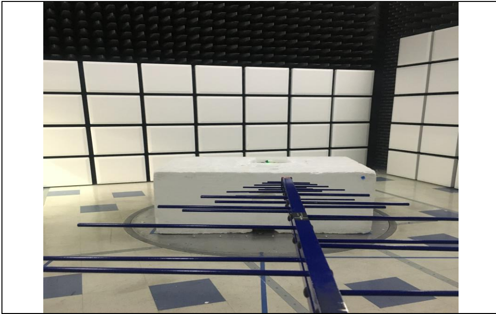
RF Radiated #1
