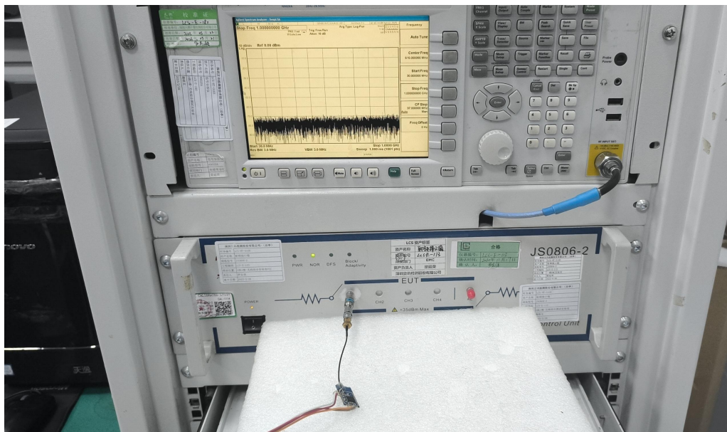
Test Setup Photo(s) of RF Conducted Measurement
