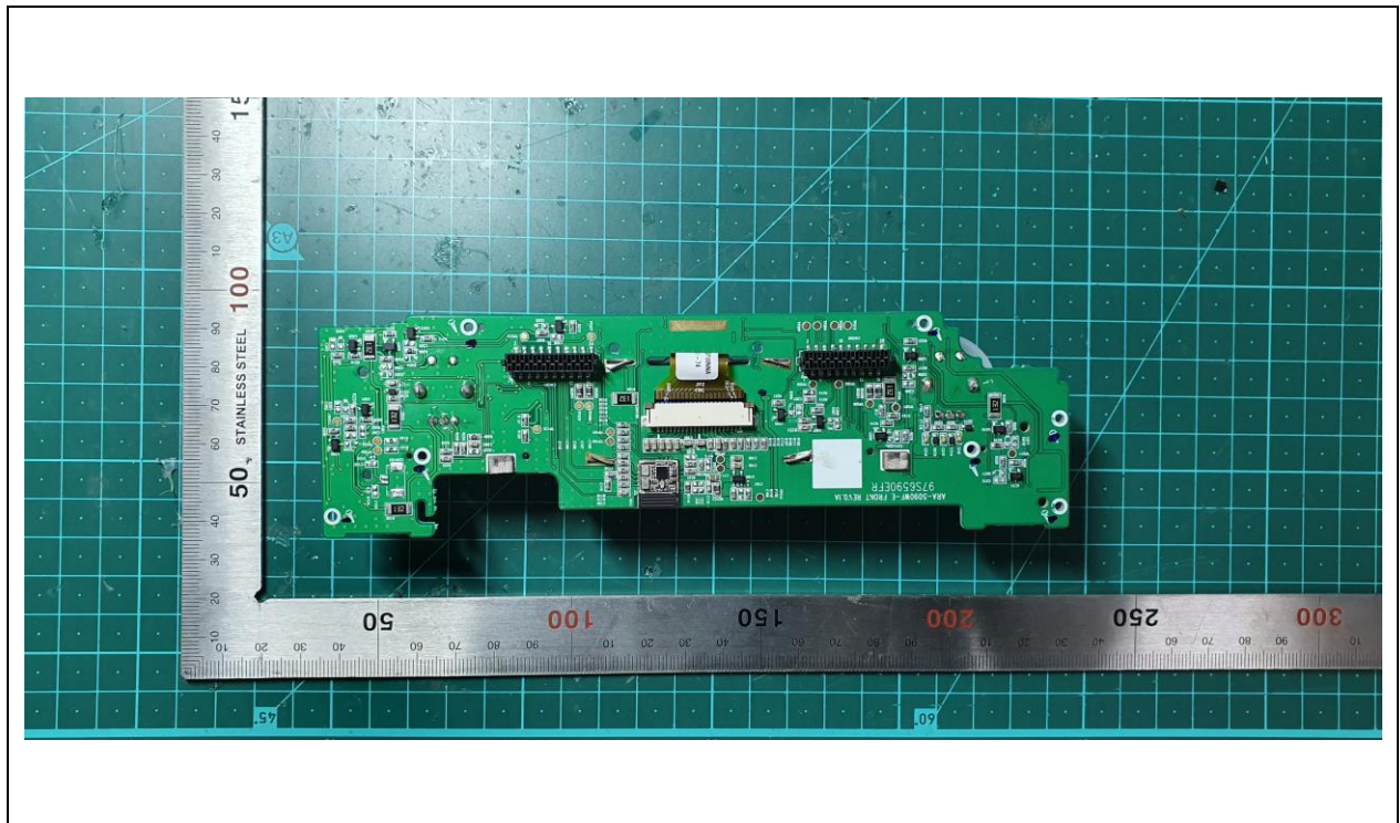
Control PCB Rear
