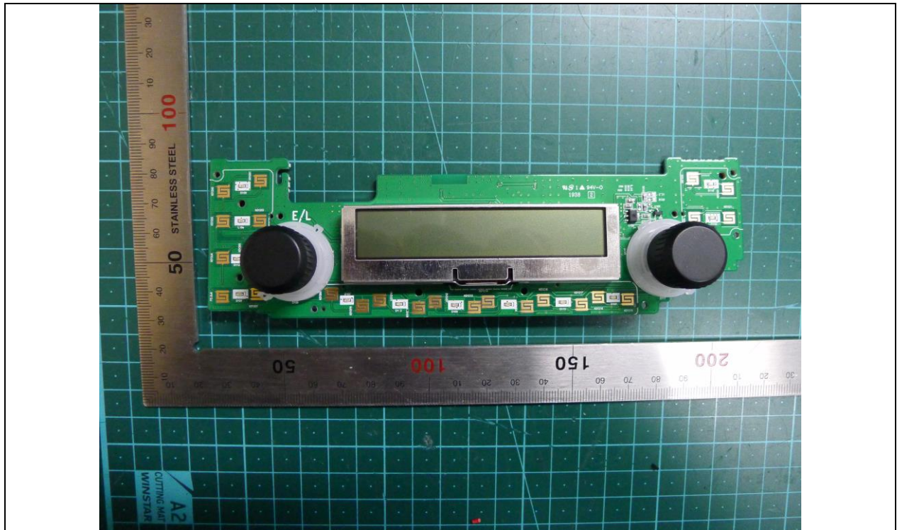
Control PCB Front
