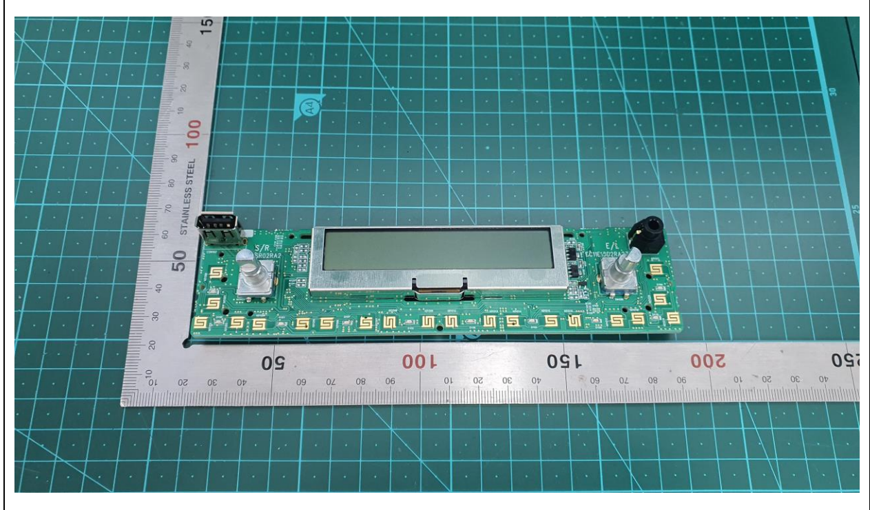
ARA-9010H Key PCB Front
