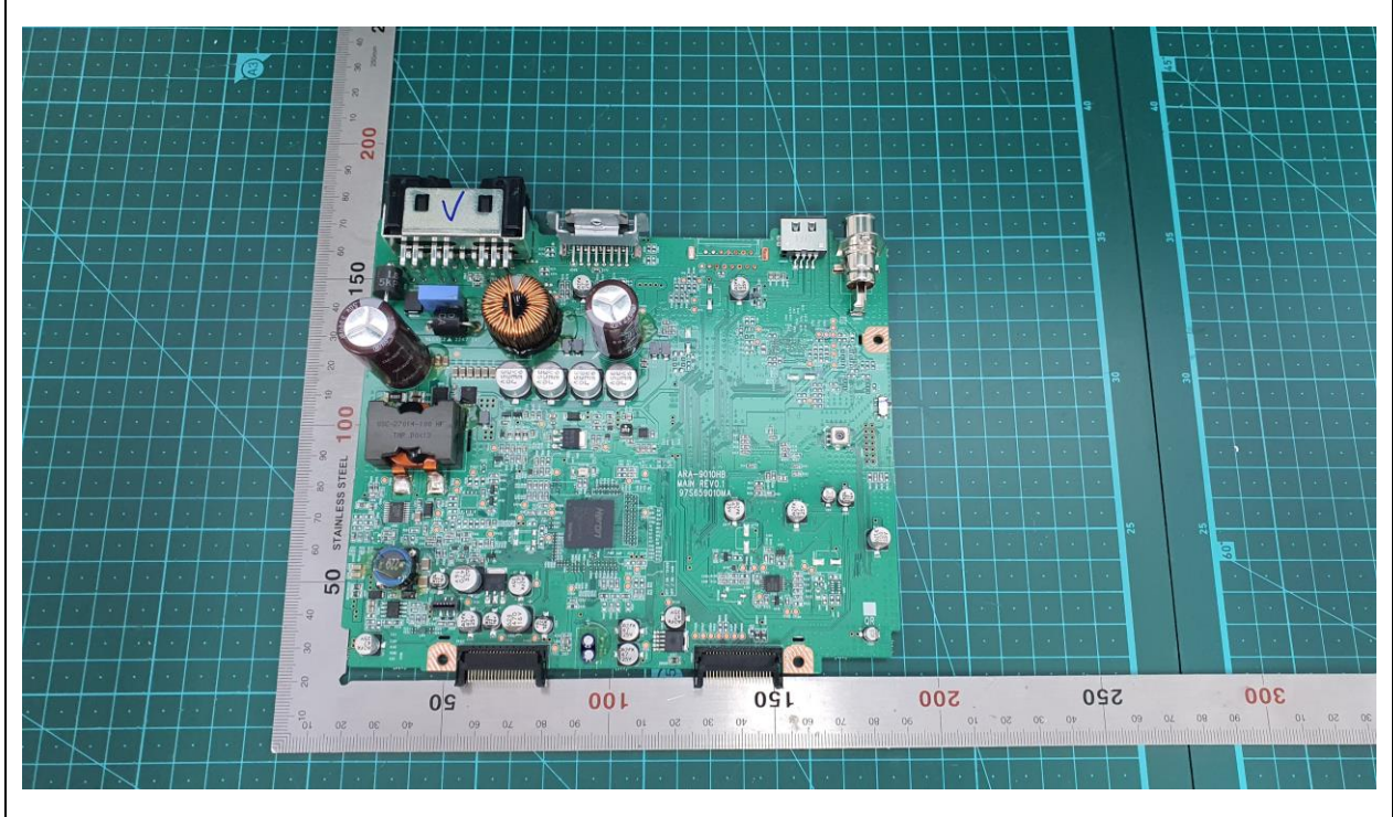
ARA-9010H Main PCB Front
