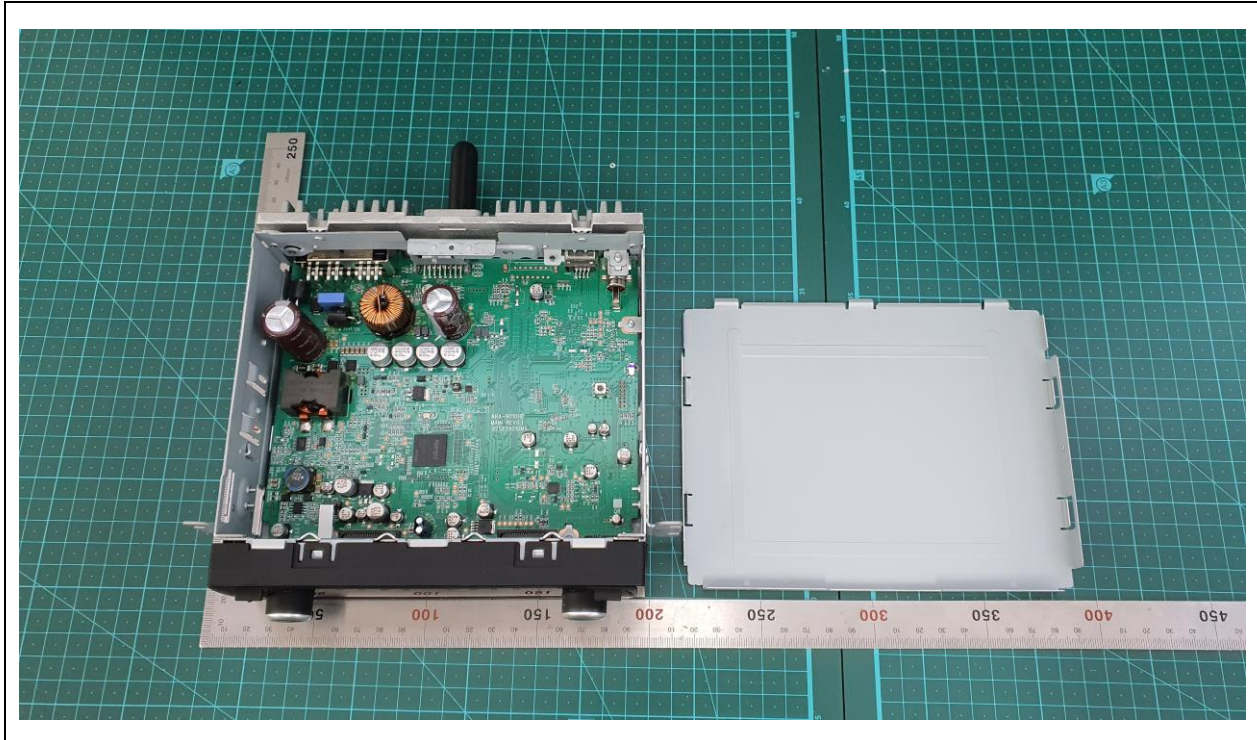
ARA-9010HB Inside
