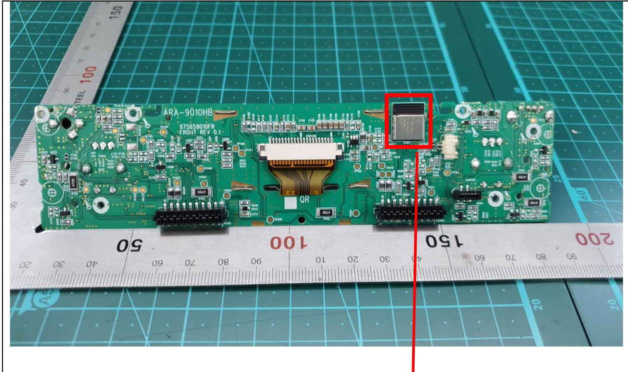
ARA-9010HB : With Bluetooth Module
