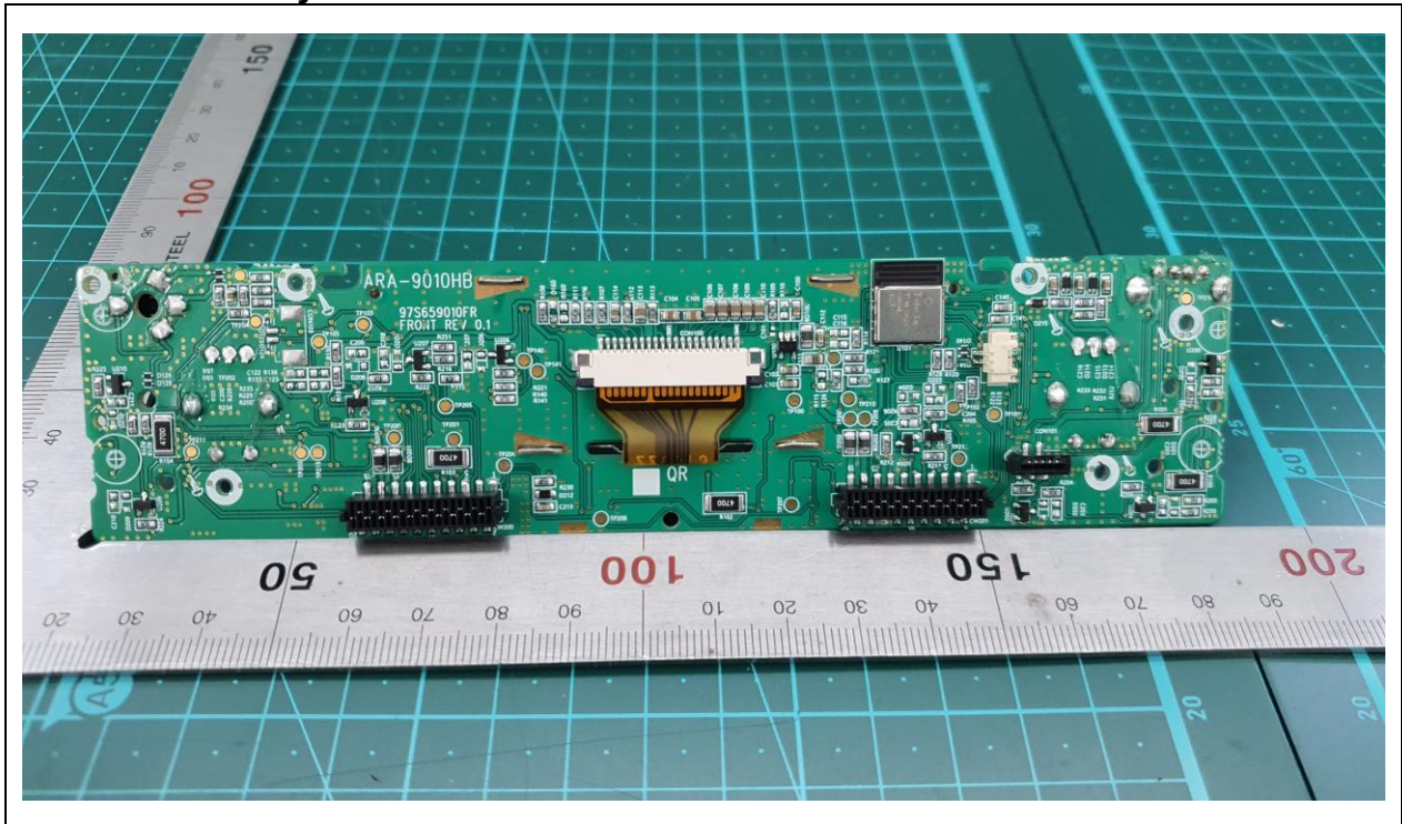
ARA-9010HB Key PCB Rear
