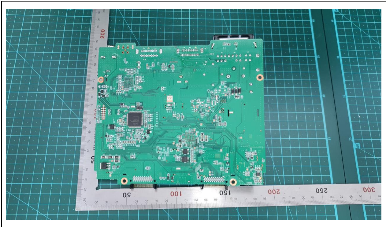
ARA-9010H Main PCB Rear
