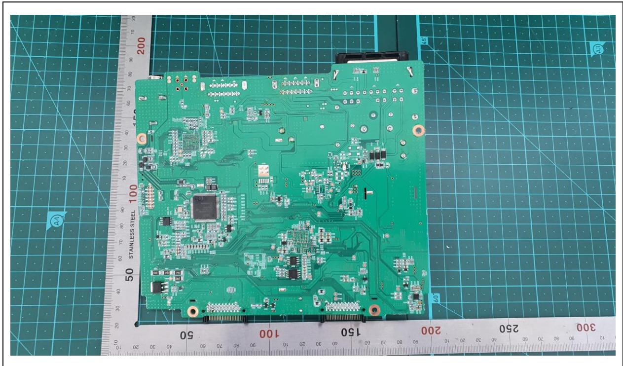
ARA-9010HB Main PCB Rear
