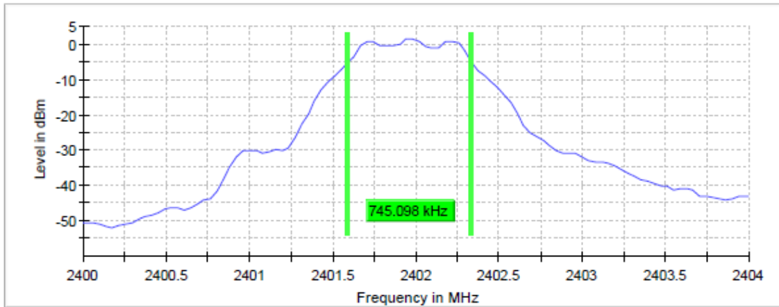
6 dB Bandwidth Plot on Configuration : 0ch
