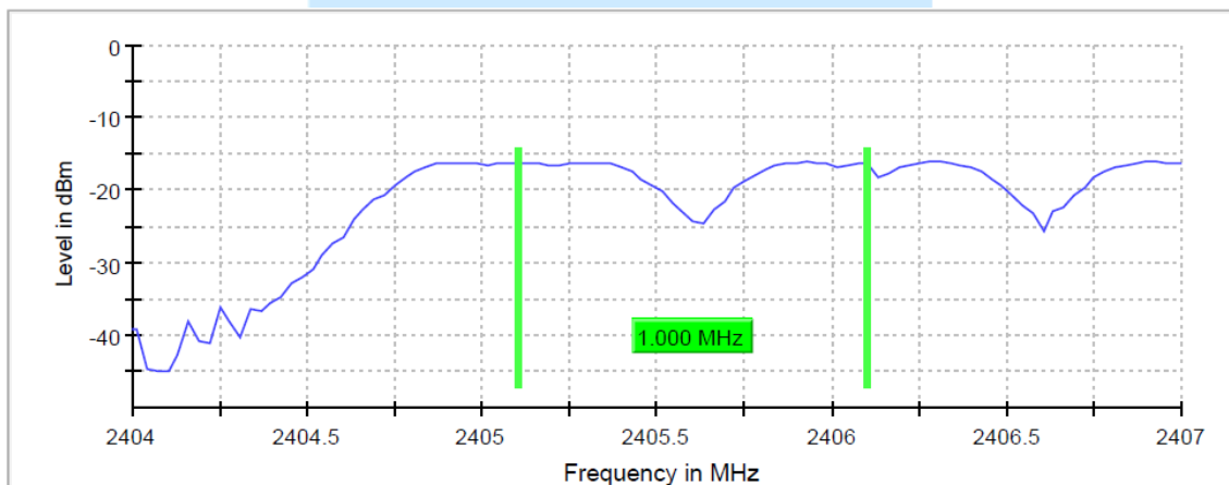
Carrier Frequency Separation Plot on configuration : 1ch
