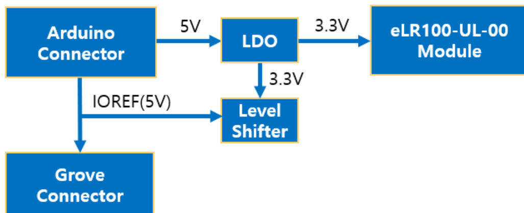
Figure 2. Power Supply
