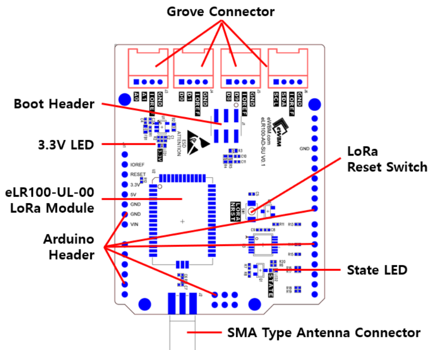
Figure 3. eLR100-AD-SU Parts
