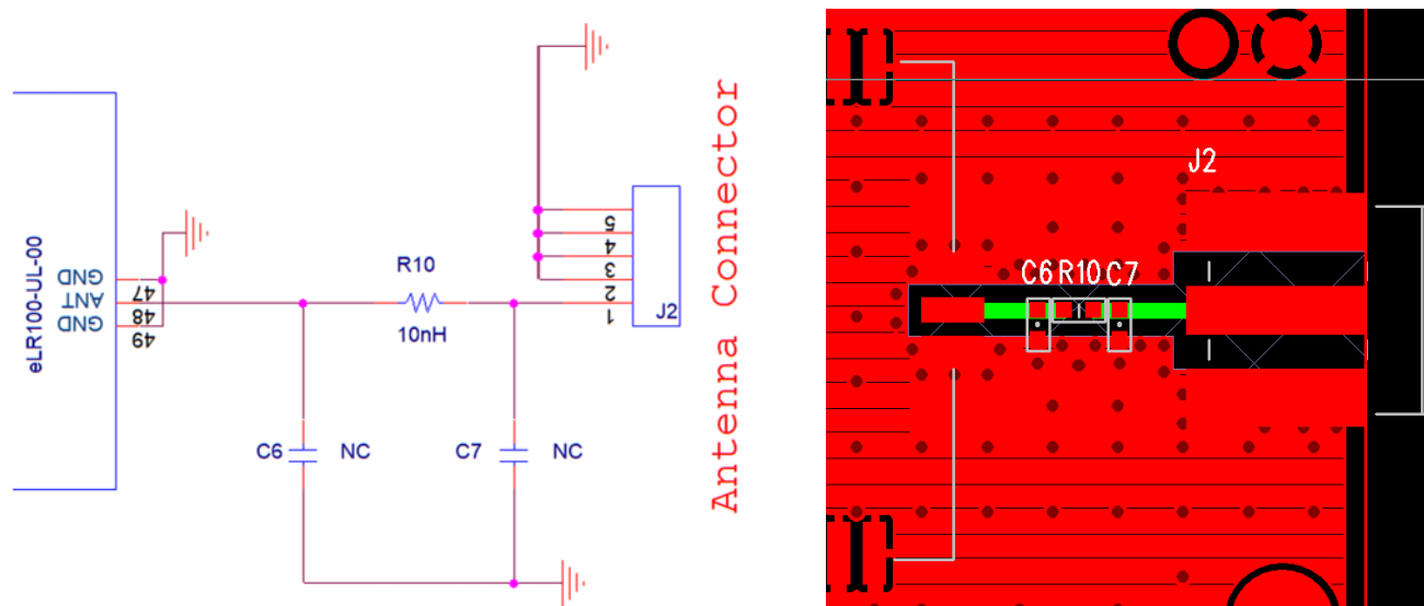
Figure 17. Antenna Reference Trace Design
