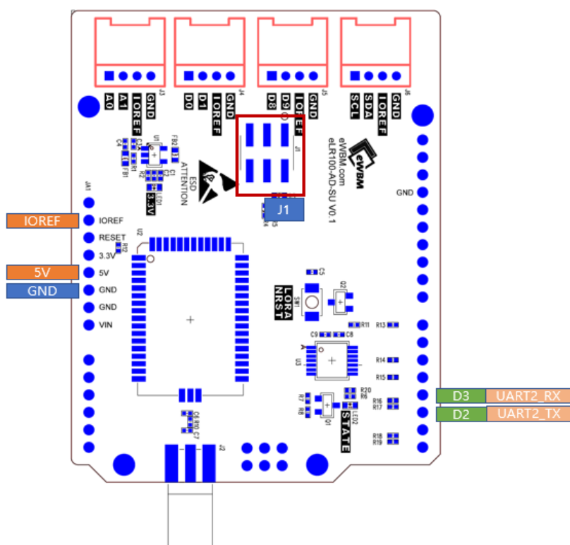
Figure 8. Boot Mode
