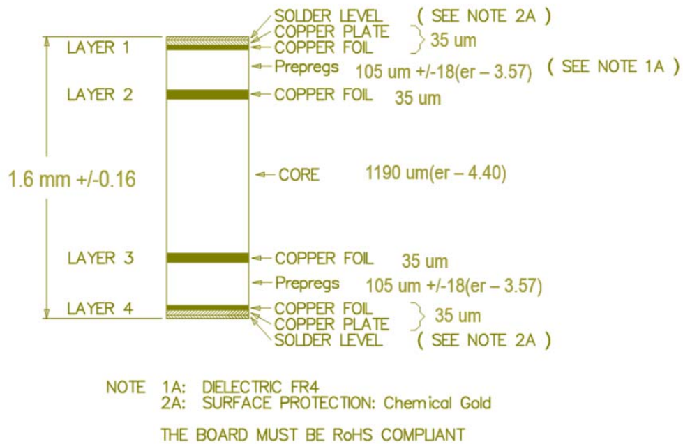
Figure 18. PCB Stack-Up
