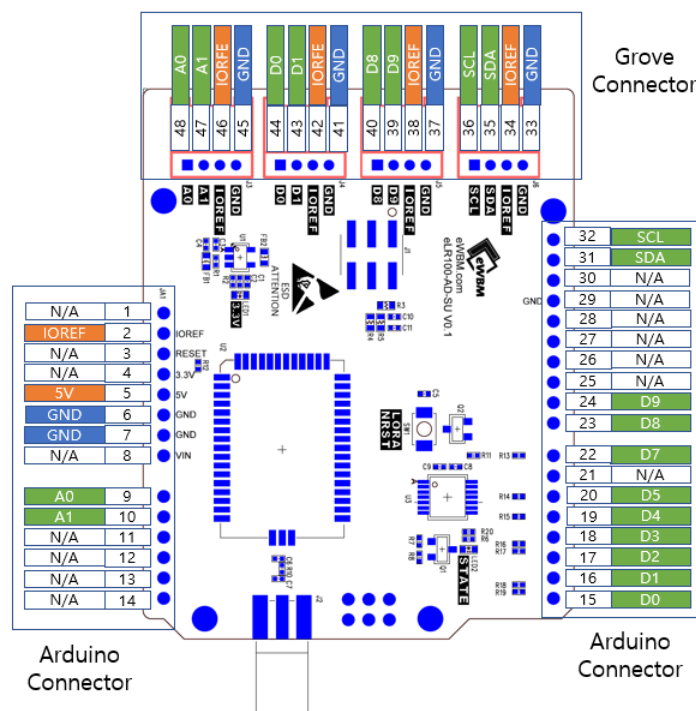
Figure 4. eLR100-AD-SU Arduino & Grove Header
