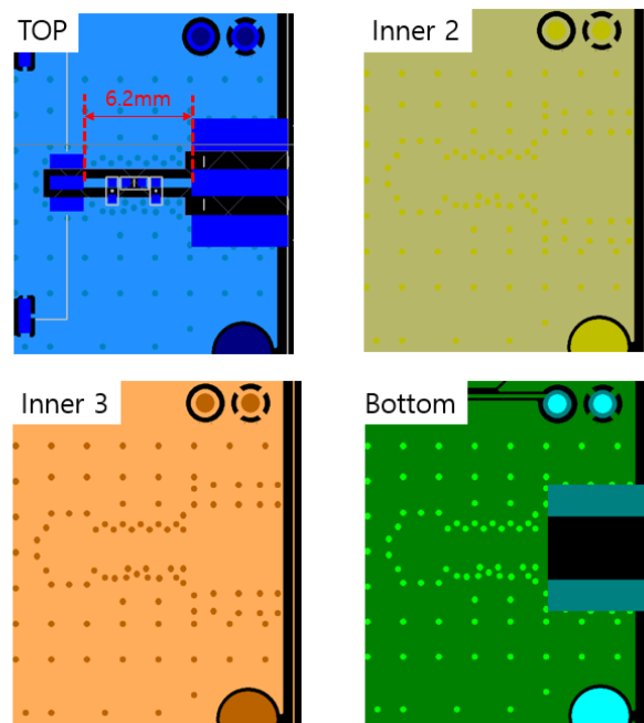
Figure 19. PCB Trace
