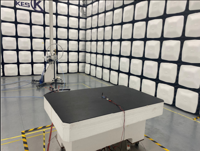
Radiated emissions
