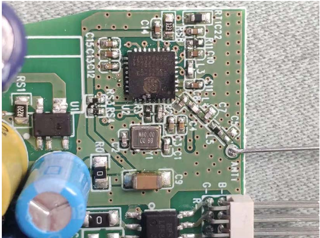
FIGURE 7 ABODE COLOR BULB (M/N: 104062/A) ANTENNA
