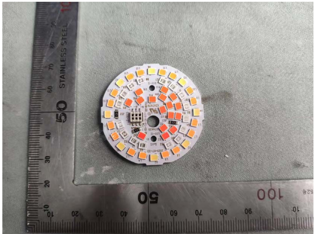
FIGURE 2 ABODE COLOR BULB (M/N: 104062/A) LED (FRONT)
