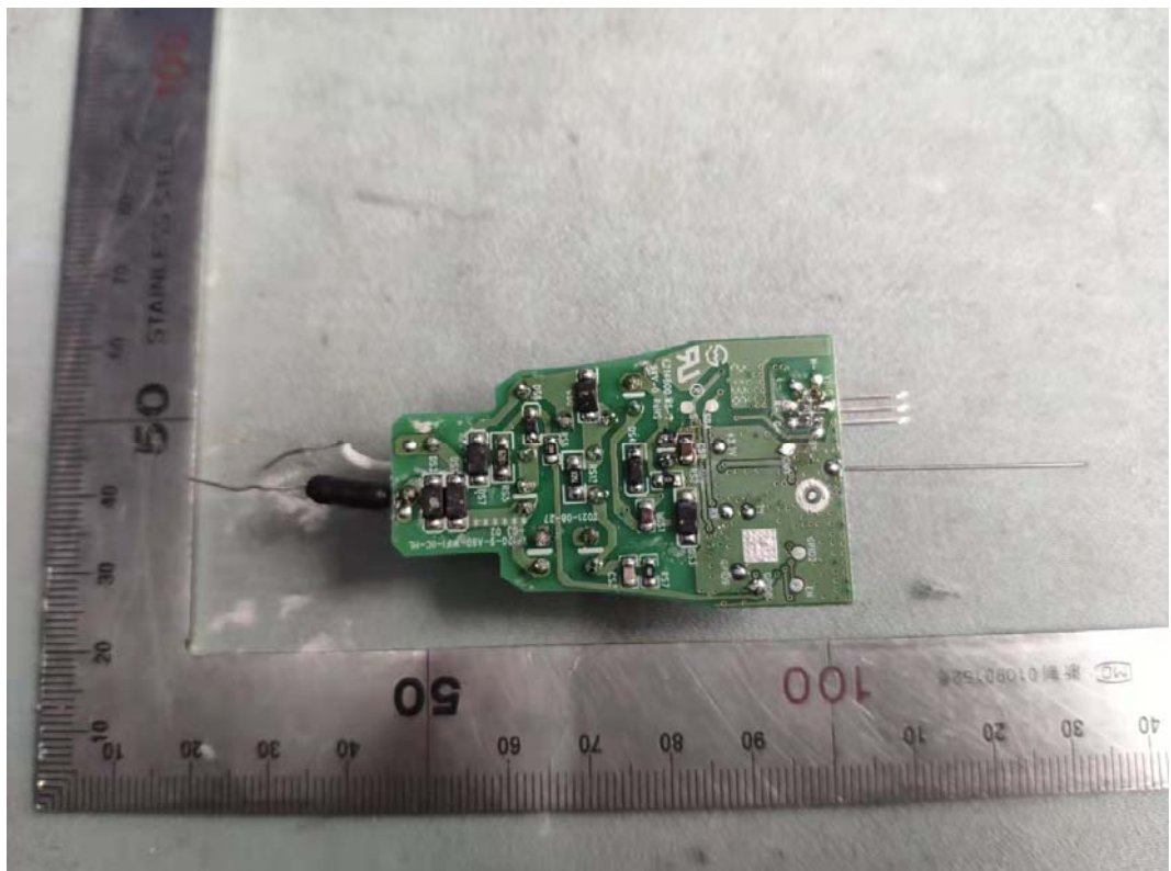
FIGURE 5 ABODE COLOR BULB (M/N: 104062/A) MAIN BOARD (SOLDERED SIDE)
