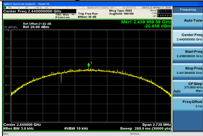
BLE_2M-Ant1-2440-PASS
