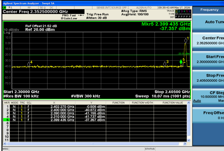
BLE_1M-Ant1-2402-PASS
