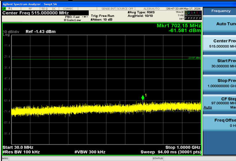
BLE_1M-Ant1-2480-30~1000-PASS
