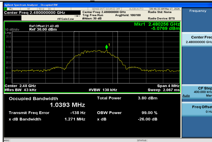
BLE_1M-Ant1-2480
