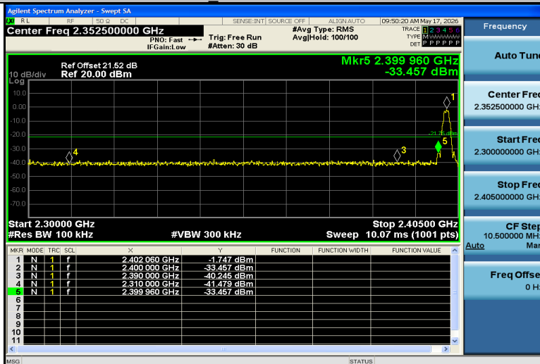
BLE_2M-Ant1-2402-PASS
