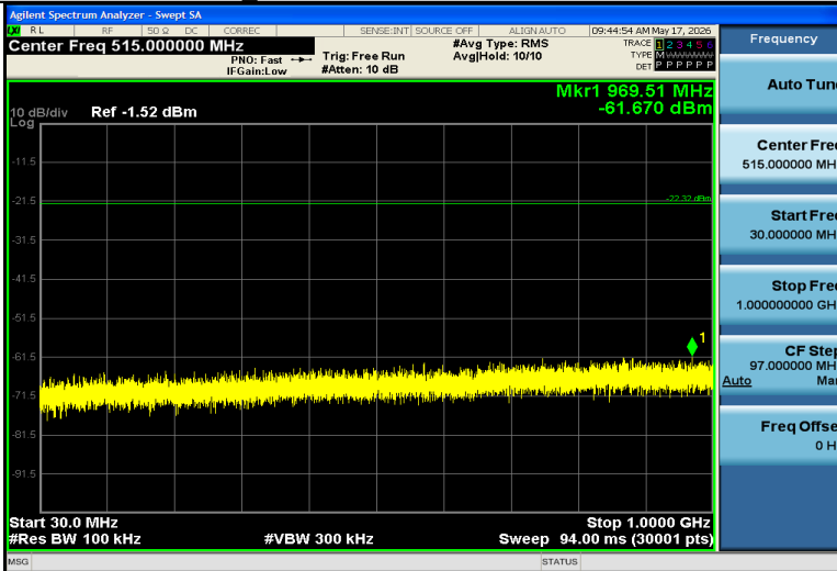
BLE_1M-Ant1-2440-30~1000-PASS
