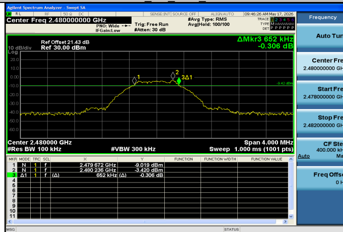
BLE_1M_Ant1_2480
