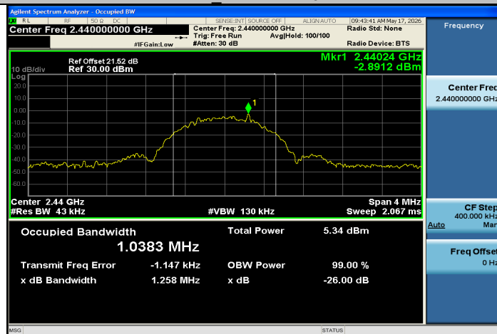
BLE_1M-Ant1-2440
