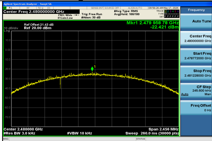
BLE_2M-Ant1-2480-PASS
