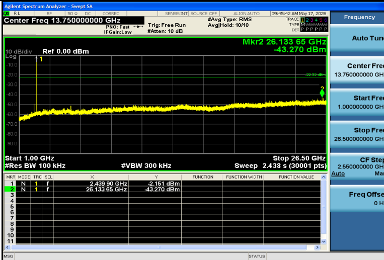
BLE_1M-Ant1-2440-1000~26500-PASS
