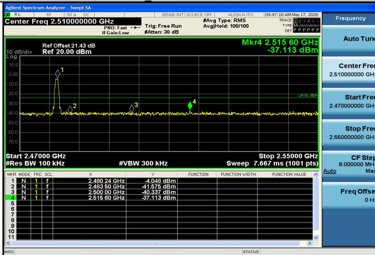
BLE_1M-Ant1-2480-PASS
