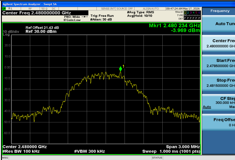
BLE_1M-Ant1-2480-0~Reference-PASS
