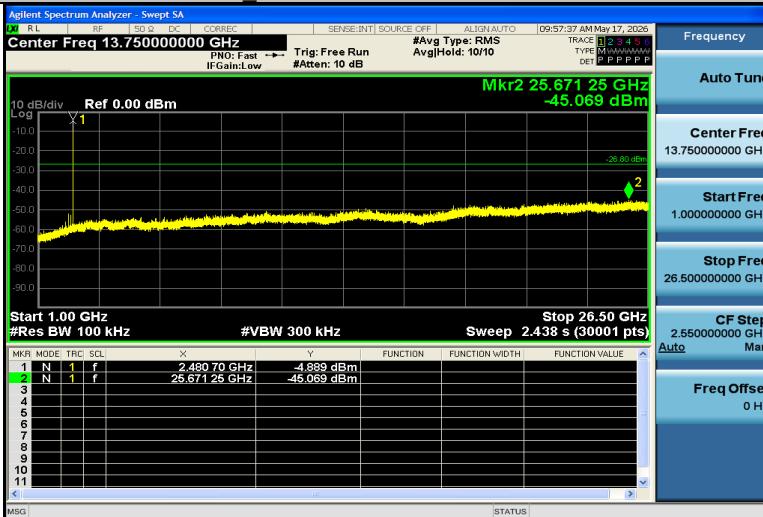
BLE_2M-Ant1-2480-1000~26500-PASS
