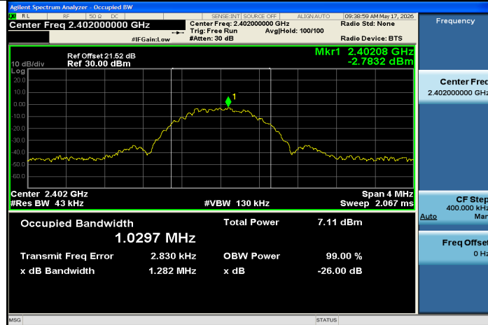
BLE_1M-Ant1-2402
