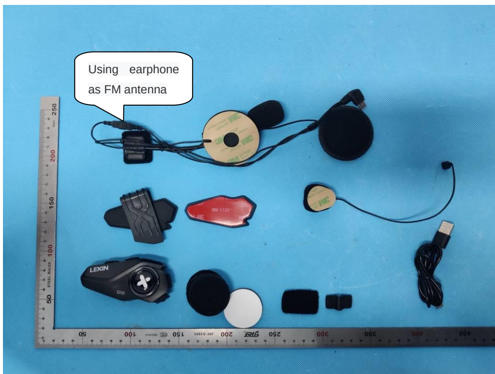
The series model is G2 WHOLE VIEW OF EUT
