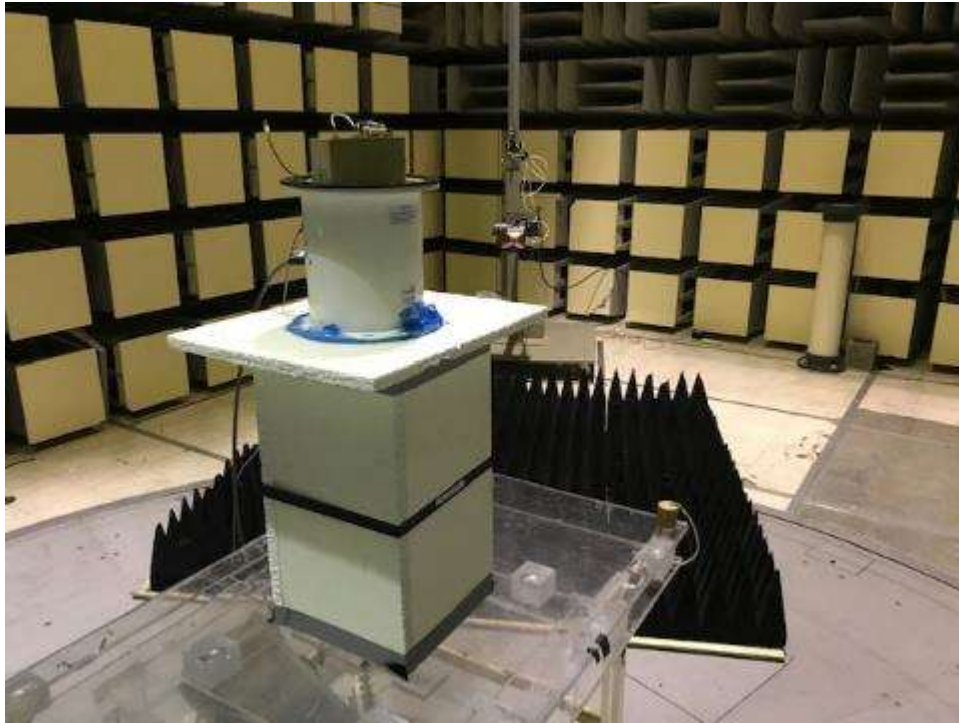
Radiated Emissions below 18 GHz.
