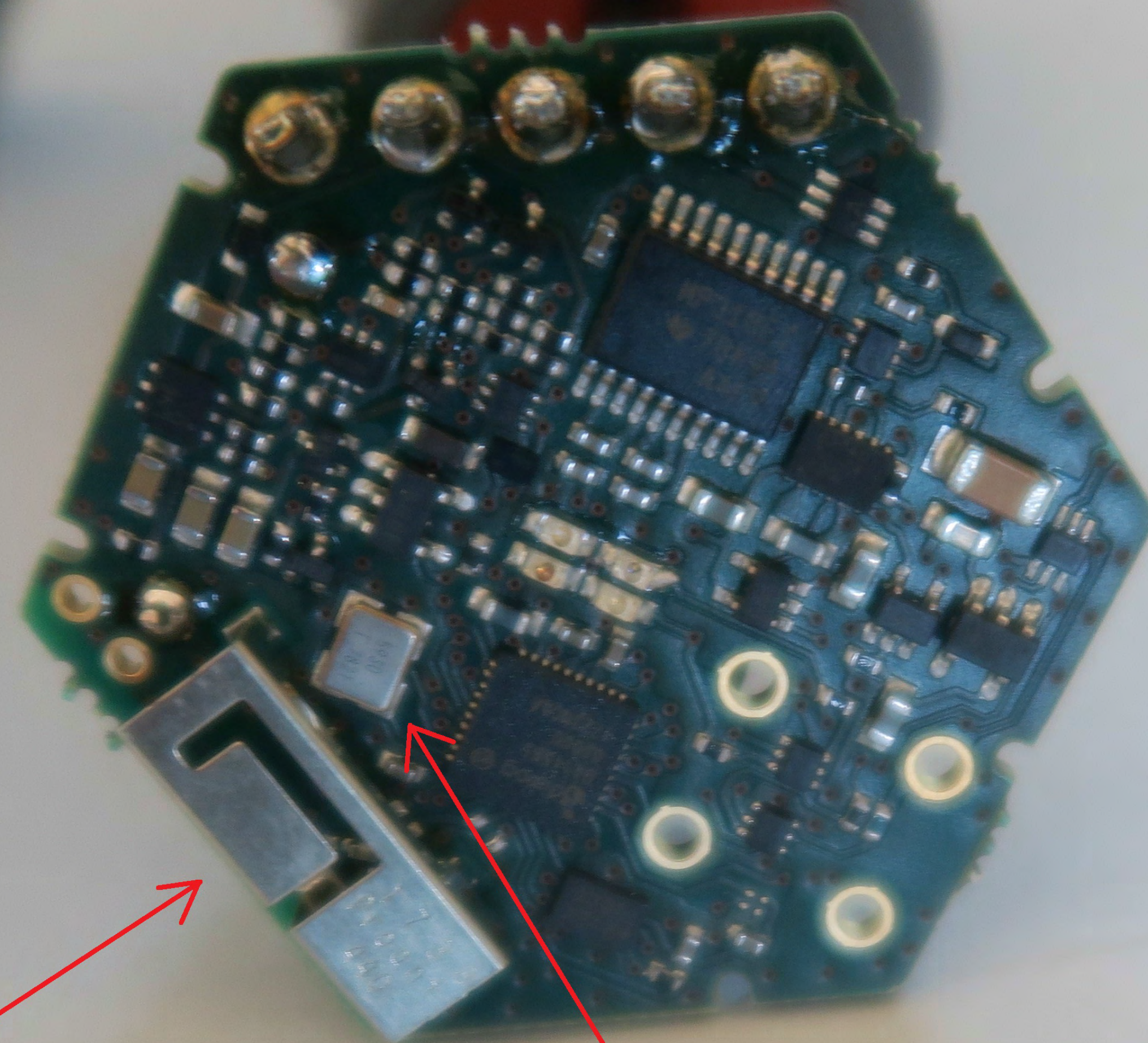
Crystal oscillator
