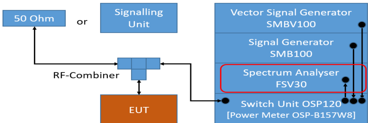
TS8997; Power Spectral Density
