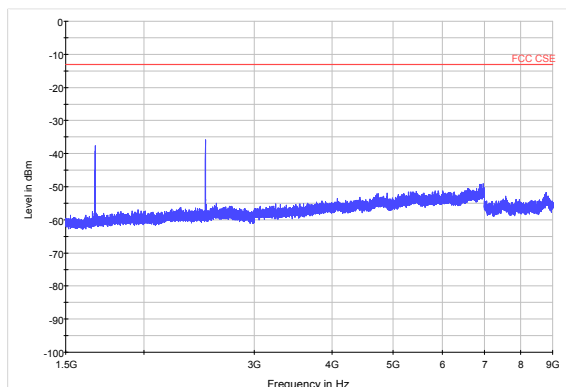
LTE Band 26 1.4MHz CH-High 1.5GHz~9GHz
