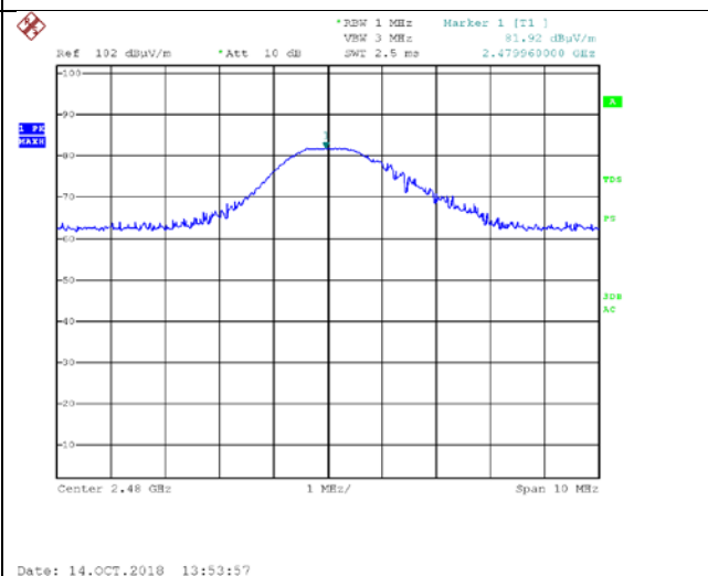
Figure 17. 2480.0 MHz, BLE, Horizontal
