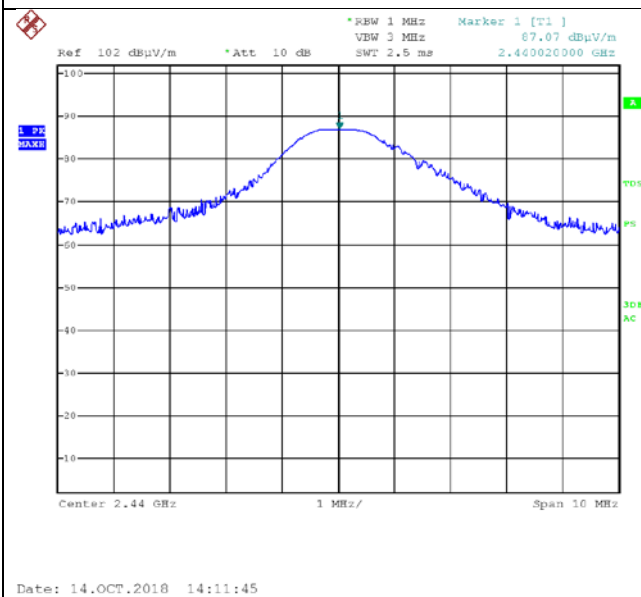
Figure 14. 2440.0 MHz, BLE, Vertical
