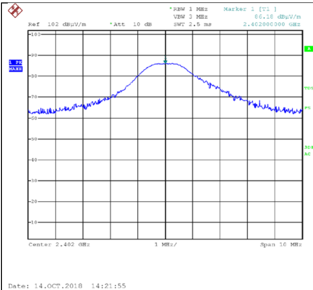
Figure 12. 2402.0 MHz, BLE, Vertical
