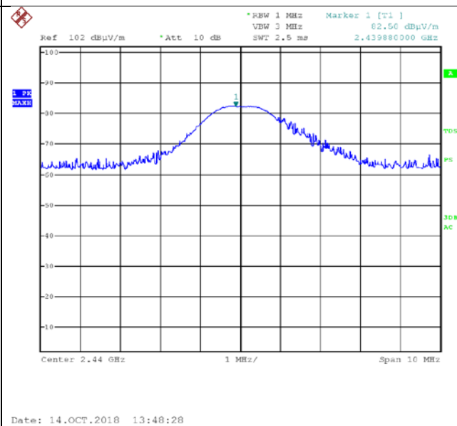
Figure 15. 2440.0 MHz, BLE, Horizontal
