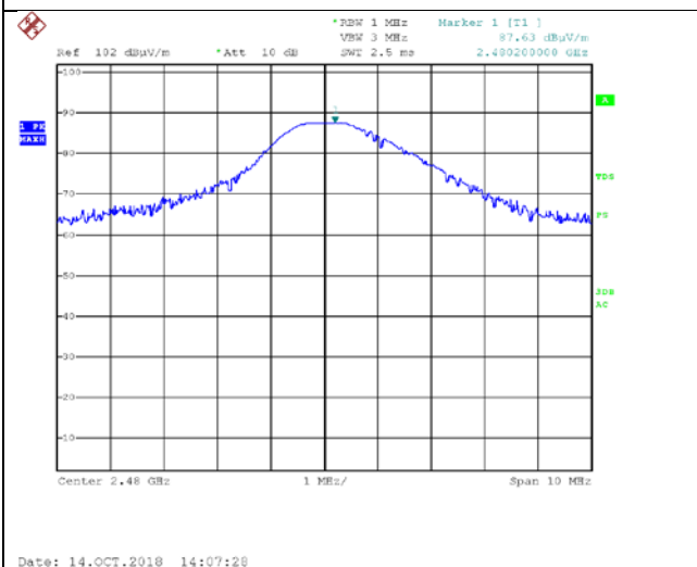
Figure 16. 2480.0 MHz, BLE, Vertical
