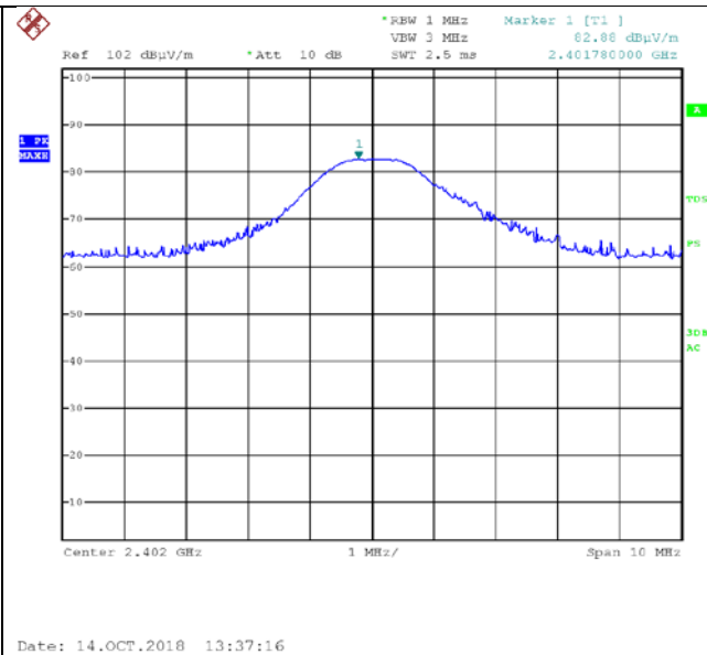
Figure 13. 2402.0 MHz, BLE, Horizontal
