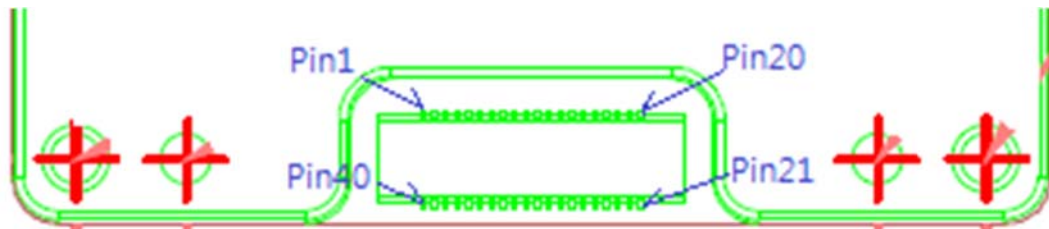
HIROSE Header DF40C-40P-0.4V(51) ( Top view )
