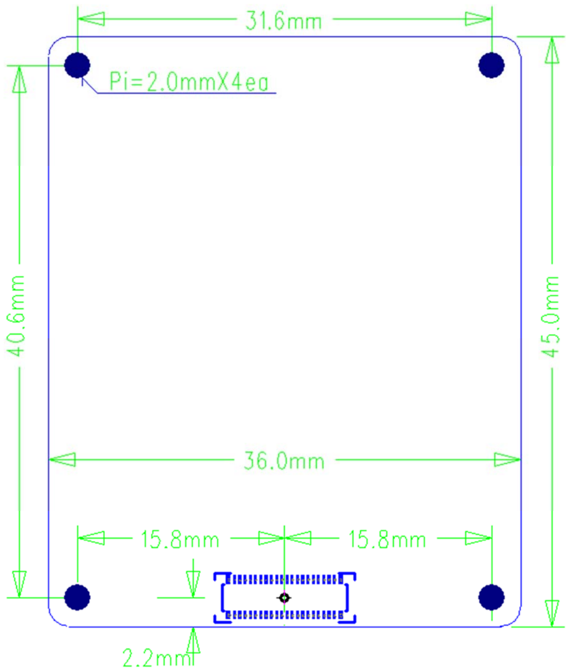
KCTM-2000 Board Dimension
