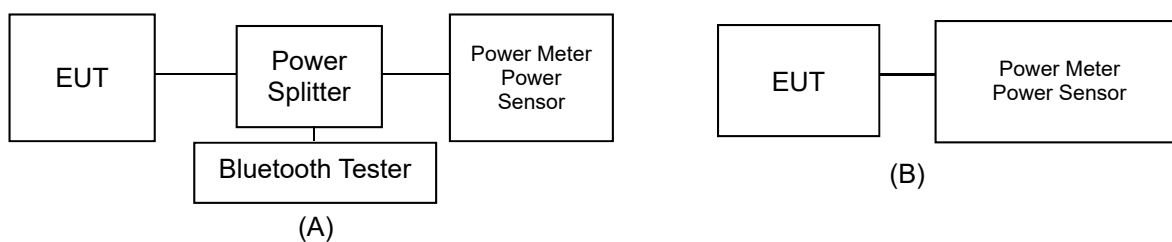
Figure 8.2.1 Average Power Measurement Setup
