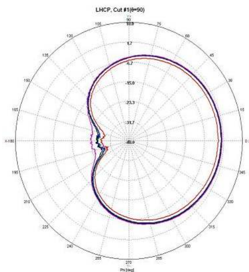
RADIATION PATTERN
