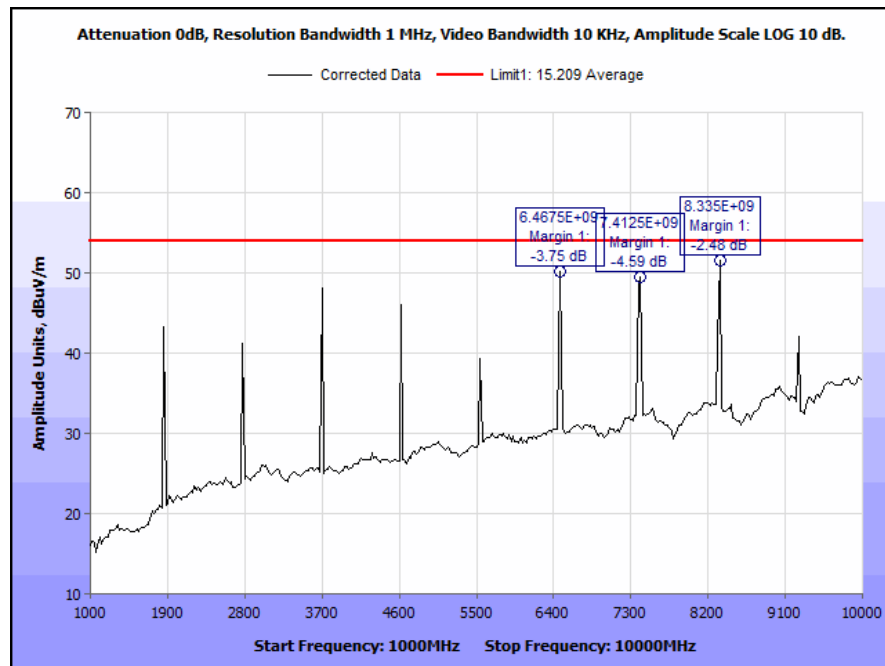
Plot 4. Radiated Spurious Emissions, 1 GHz – 10 GHz, Average
