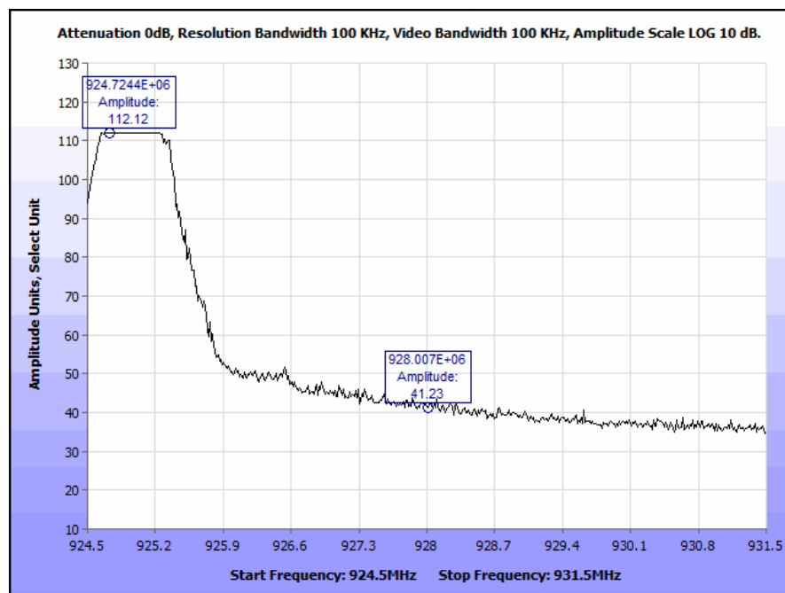
Plot 10. Radiated Restricted Band Edge, High Channel
