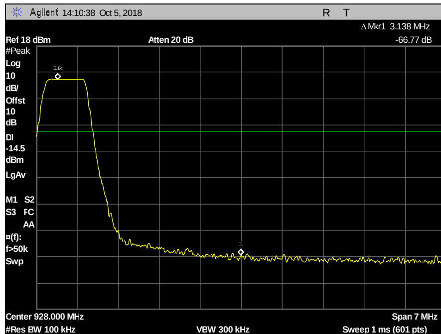
Plot 13. Conducted Band Edge, High Channel
