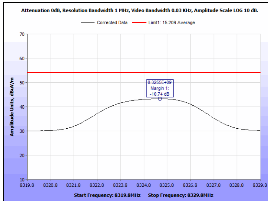
Plot 8. Radiated Spurious Emissions, 8.325 GHz Spur
