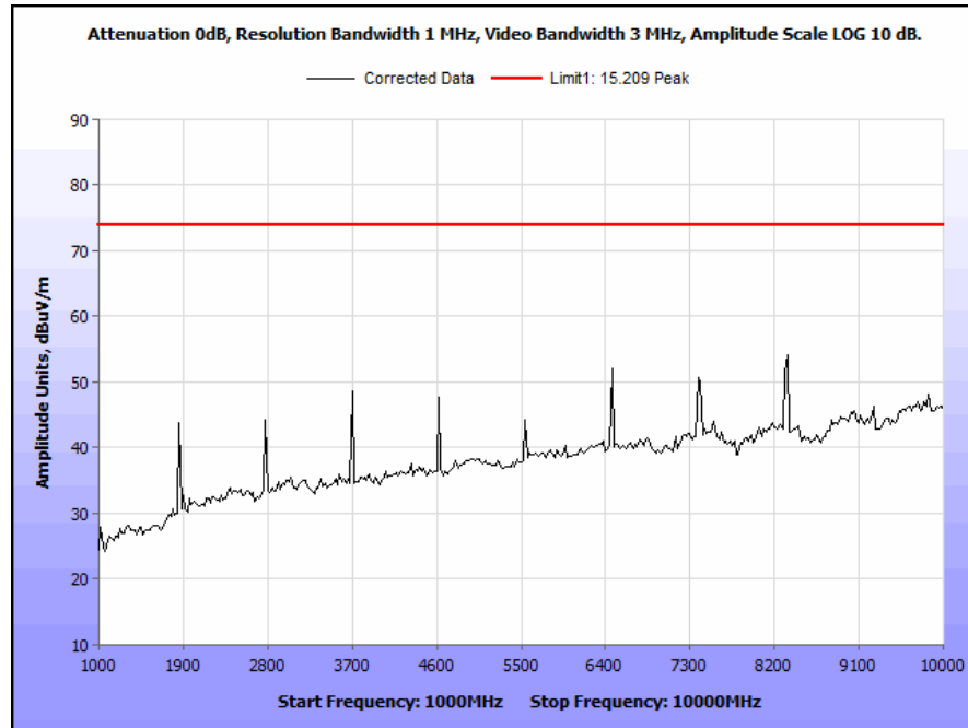
Plot 5. Radiated Spurious Emissions, 1 GHz – 10 GHz, Peak
