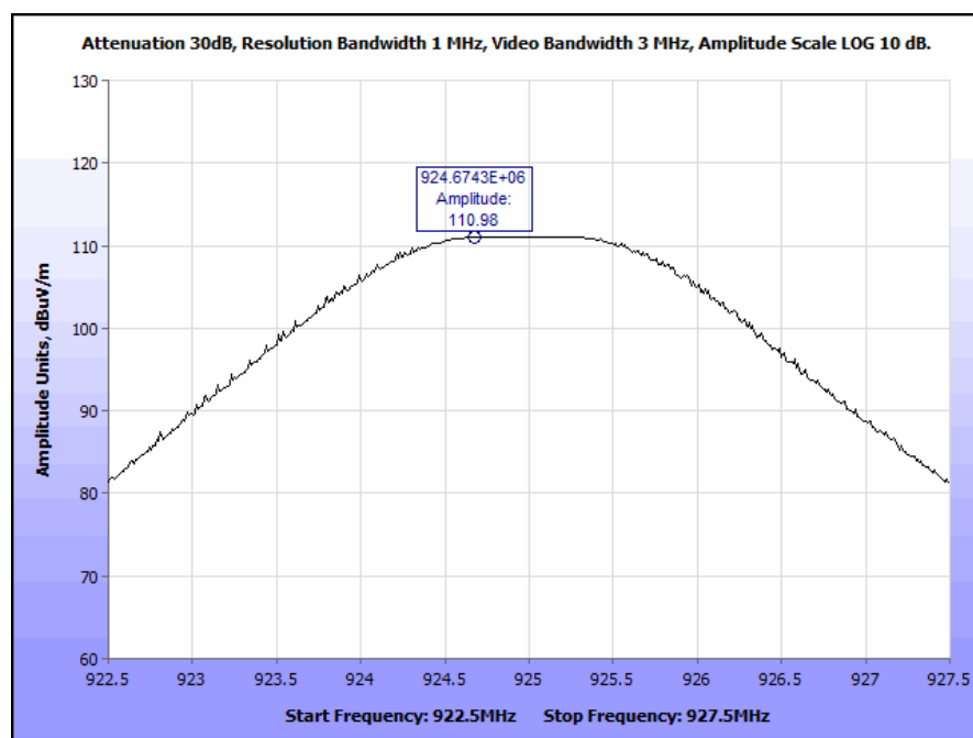
Plot 2. Peak Power Output, EIRP
