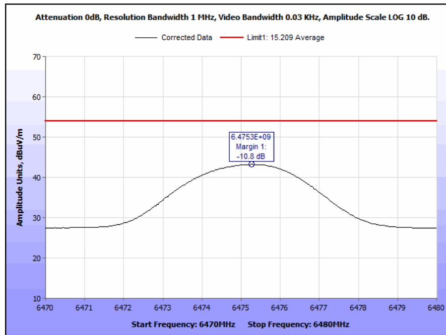
Plot 6. Radiated Spurious Emissions, 6.475 GHz Spur
