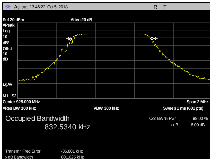
Plot 1. 6 dB Occupied Bandwidth, 925 MHz
