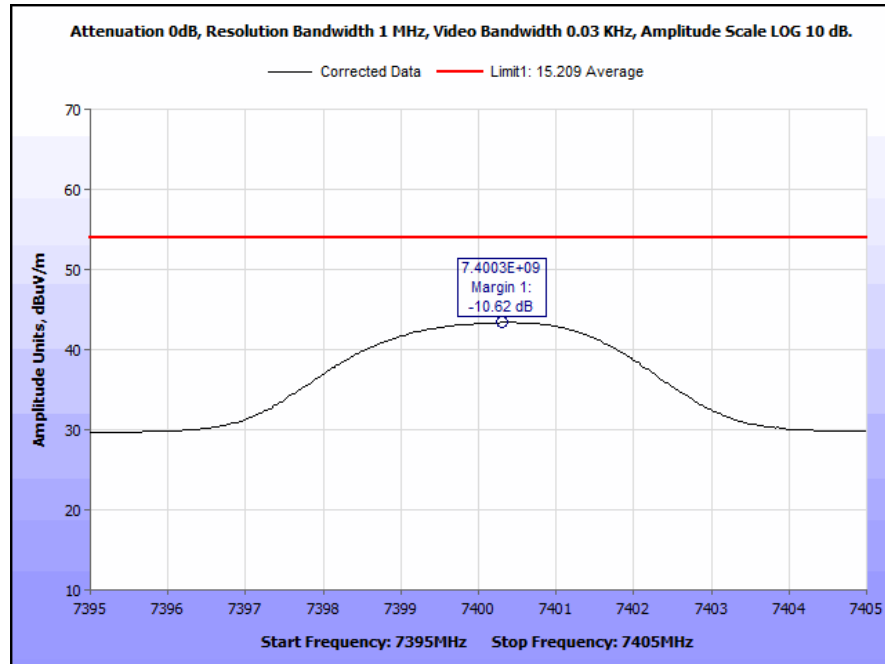
Plot 7. Radiated Spurious Emissions, 7.4 GHz Spur
