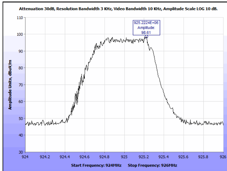
Plot 14. Peak Power Spectral Density, Radiated Measurement
