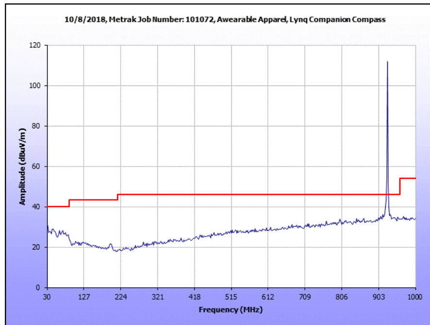
Plot 3. Radiated Spurious Emissions, 30 MHz – 1 GHz
