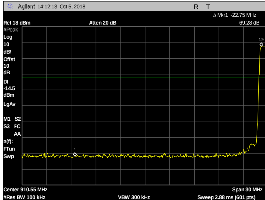
Plot 12. Conducted Band Edge, Low, Channel
