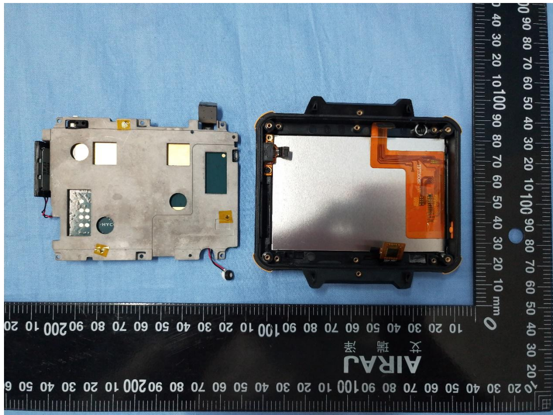
6. Smart Watch uncover view
