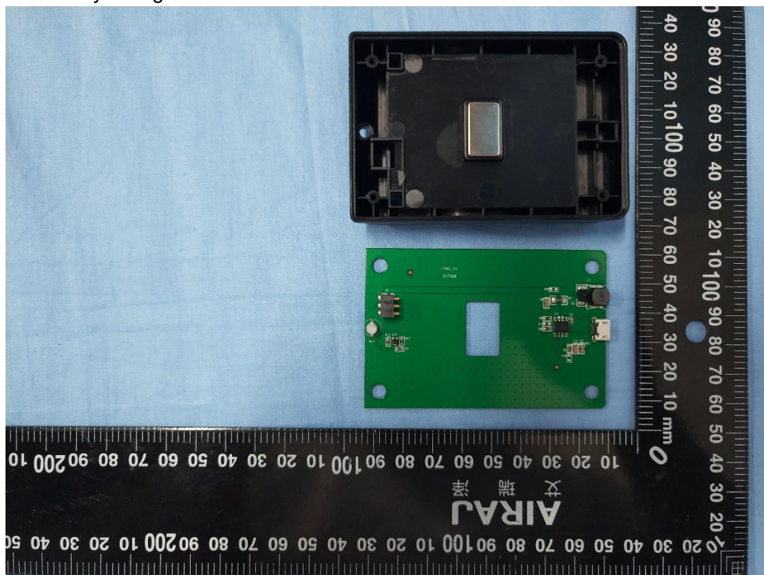
14. Battery Charger uncover view
