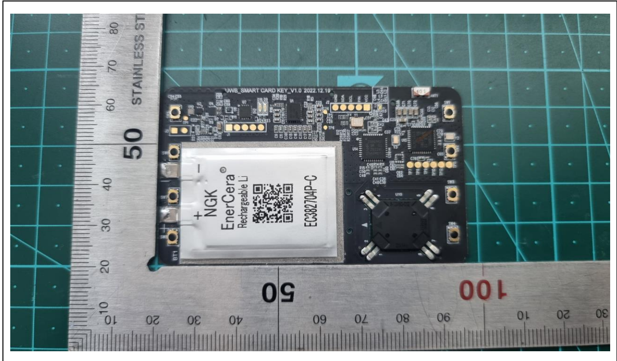
PCB Front
