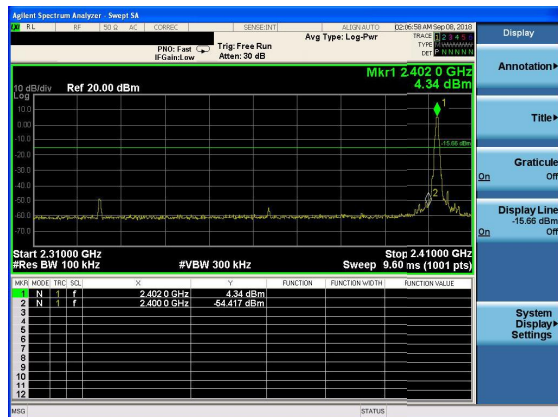
GFSK: Band Edge-Low Channel (Hopping Mode)
