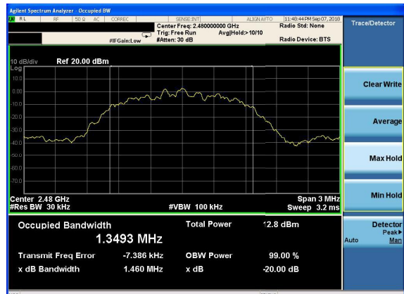
20dB Bandwidth plot on channel 78 (2Mbps)
