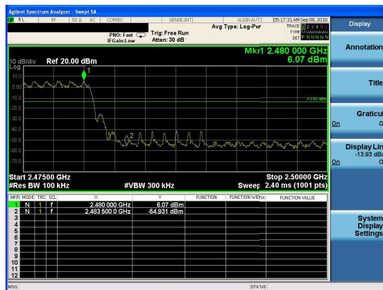
\pi/4 -DQPSK: Band Edge-High Channel (Hopping Mode)
