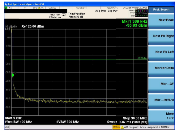
8-DPSK on channel 39
