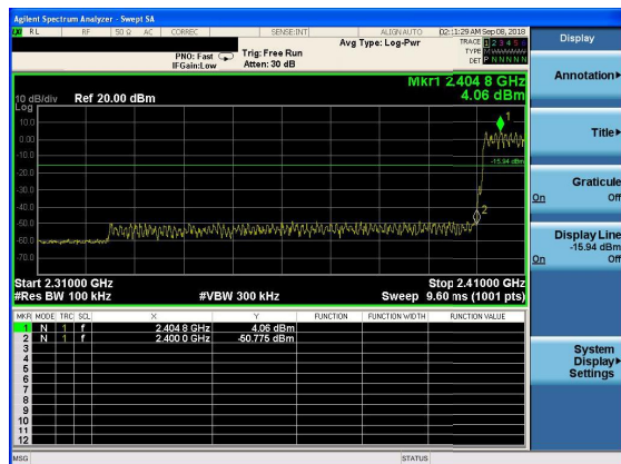
8-DPSK: Band Edge-Low Channel (Hopping Mode)
