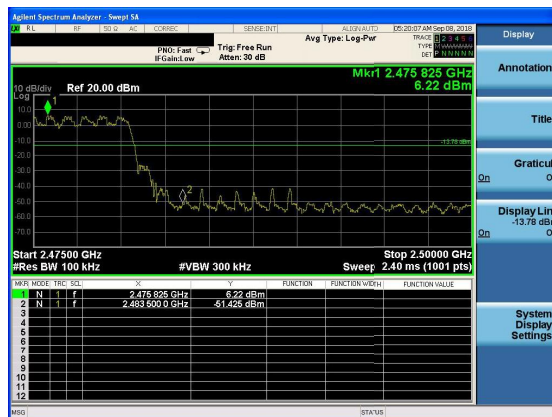
8-DPSK: Band Edge-High Channel (Hopping Mode)
