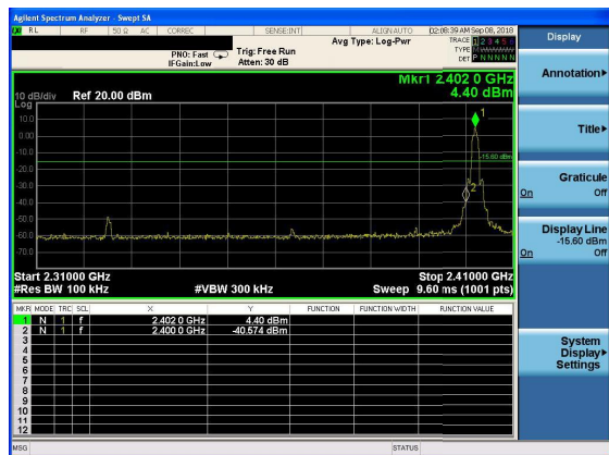
\pi/4 -DQPSK: Band Edge-Low Channel (Hopping Mode)
