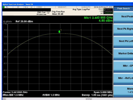
Peak output Power plot on channel 39 (1Mbps)
