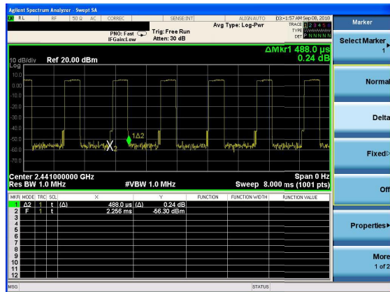
Package Transfer Time Plot CH39-3DH3
