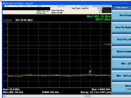
8-DPSK on channel 39
