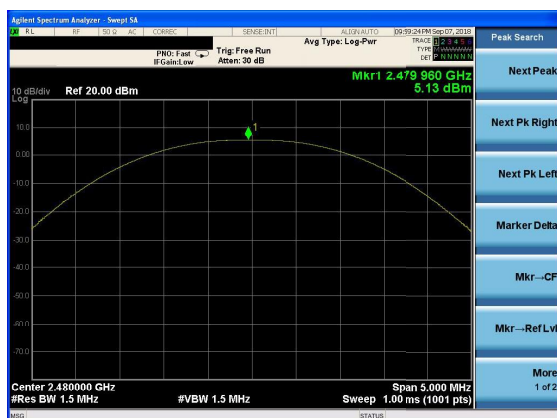
Peak output Power plot on channel 78 (1Mbps)
