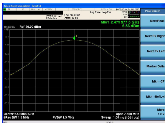
Peak output Power plot on channel 78 (3Mbps)
