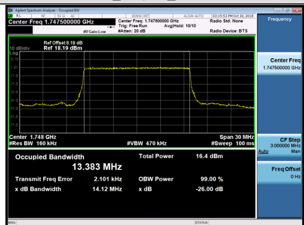
HCH_16QAM_75RB#0
