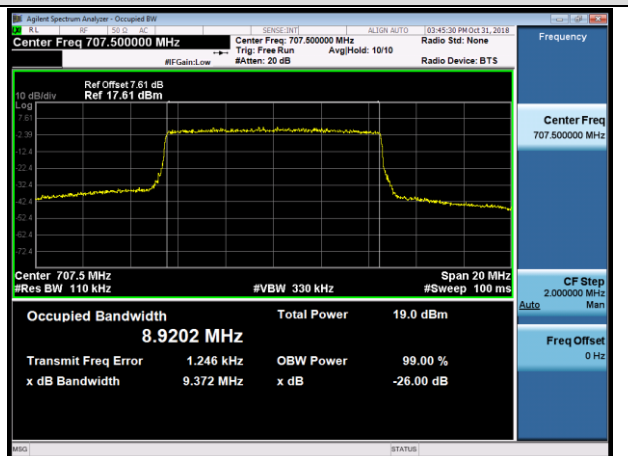
MCH_16QAM_50RB#0
