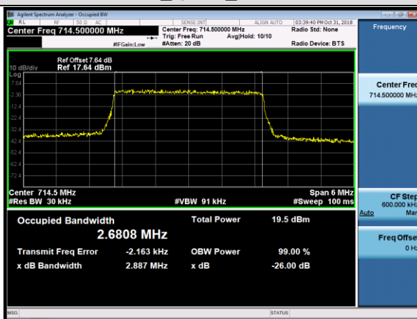
HCH_QPSK_15RB#0
