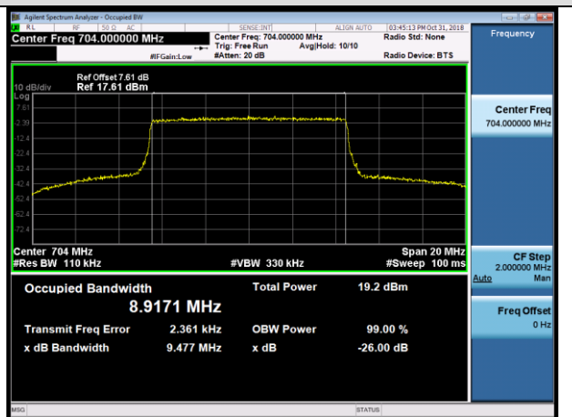
LCH_16QAM_50RB#0
