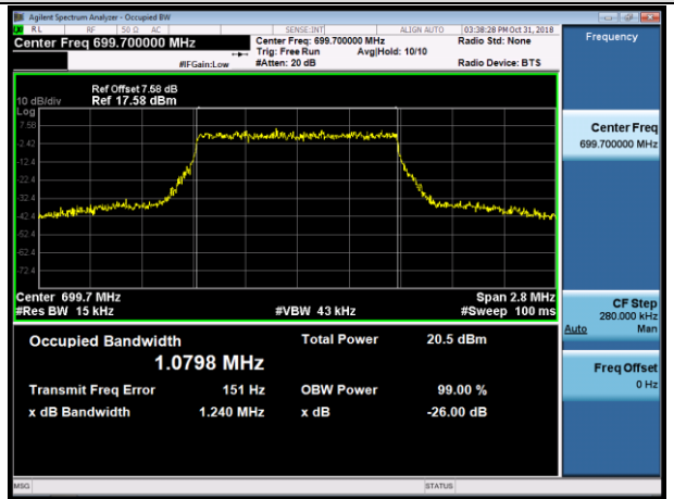
LCH_16QAM_6RB#0
