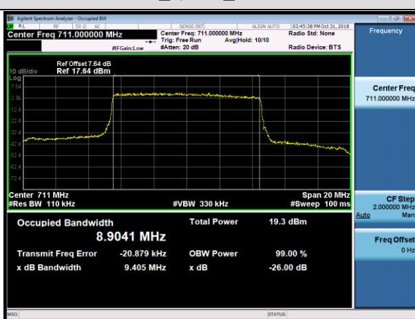
HCH_QPSK_50RB#0
