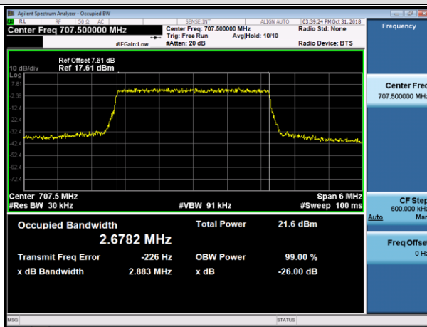
MCH_QPSK_15RB#0
