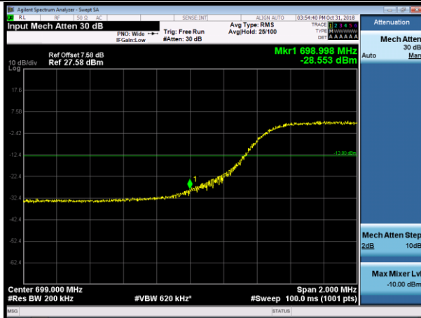
LCH_QPSK_50RB#0
