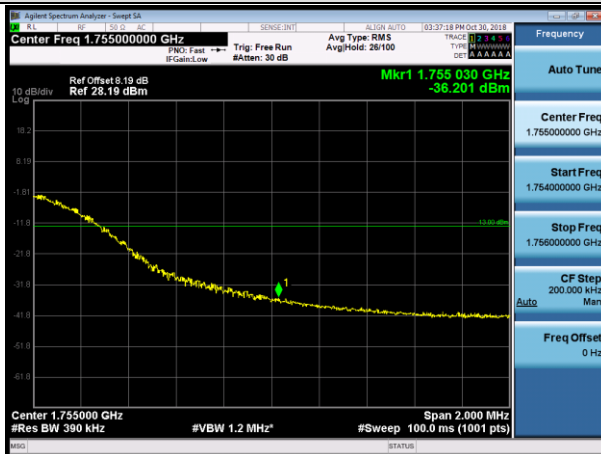
HCH_QPSK_100RB#0
