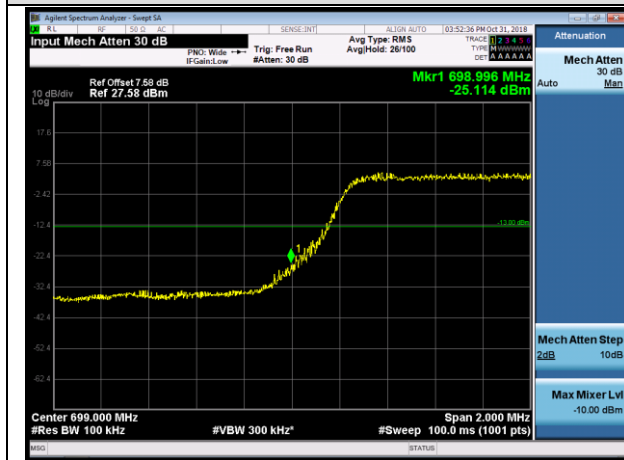
LCH_QPSK_25RB#0
