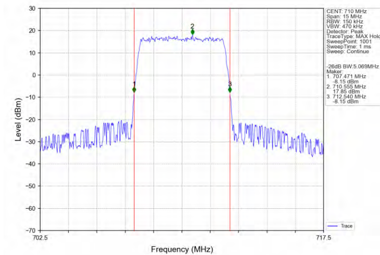
Band17_5MHz_QPSK_MCH_710MHz_RB_25_0_NTNV
