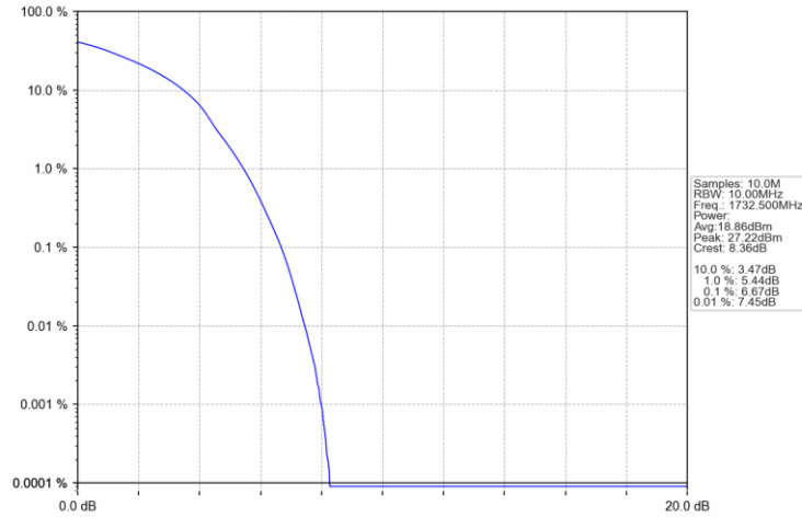
Band4_20MHz_16QAM_MCH_1732.5MHz_RB_100_0_NTNV
