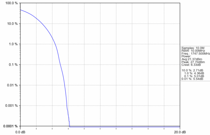
Band4_15MHz_QPSK_HCH_1747.5MHz_RB_75_0_NTNV
