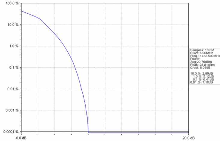
Band4_5MHz_16QAM_MCH_1732.5MHz_RB_25_0_NTNV
