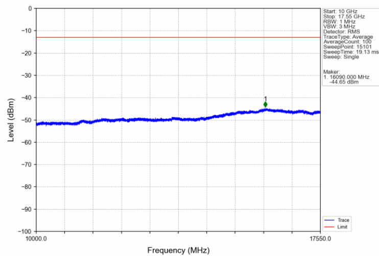
Band4_15MHz_16QAM_HCH_1747.5MHz_RB_1_0_NTNV
