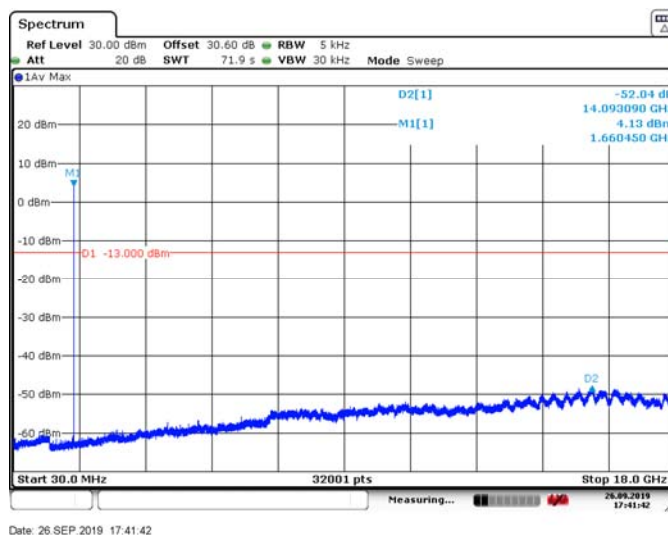
Figure 8.3-3: Spurious E. at Antenna Terminals H. channel (QPSK)
