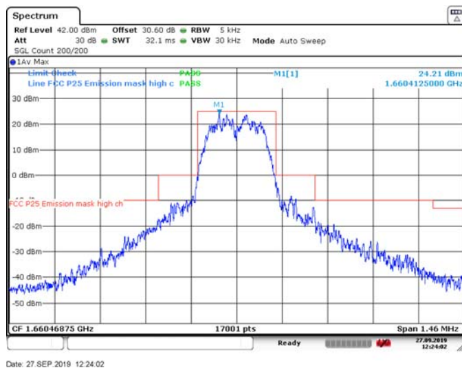
Figure 8.3-6: Emissions Mask H. channel (QPSK)
