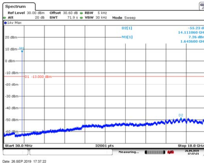
Figure 8.3-2: Spurious E. at Antenna Terminals M. channel (QPSK)
