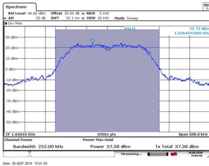
Figure 8.2-1: Power on low channel (QPSK)
