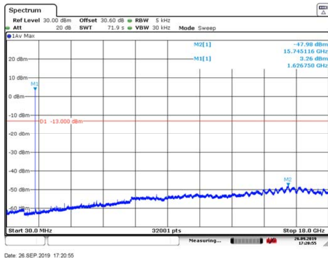
Figure 8.3-1: Spurious E. at Antenna Terminals L. channel (QPSK)
