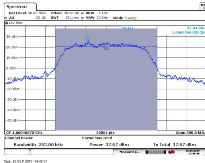
Figure 8.2-3: 99 % Power on high channel (QPSK)
