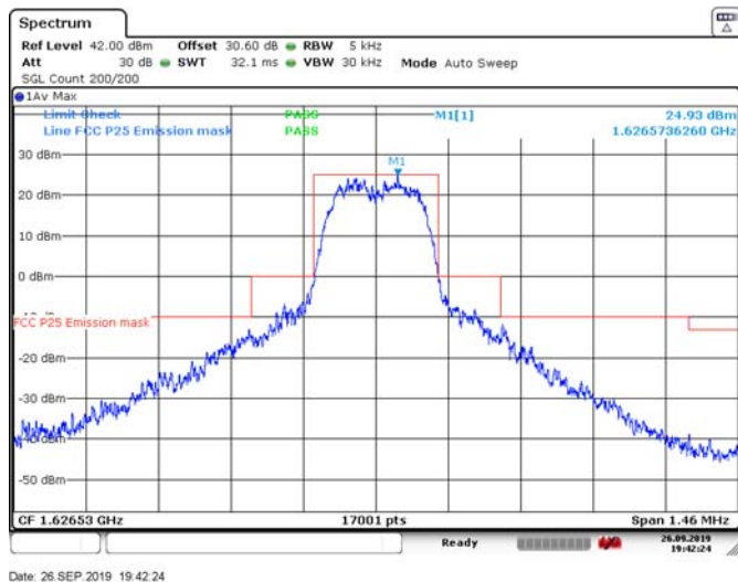
Figure 8.3-4: Emissions Mask L. channel (QPSK)
