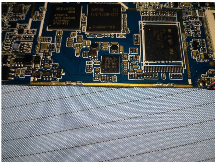
EUT – Main Chip View 1
