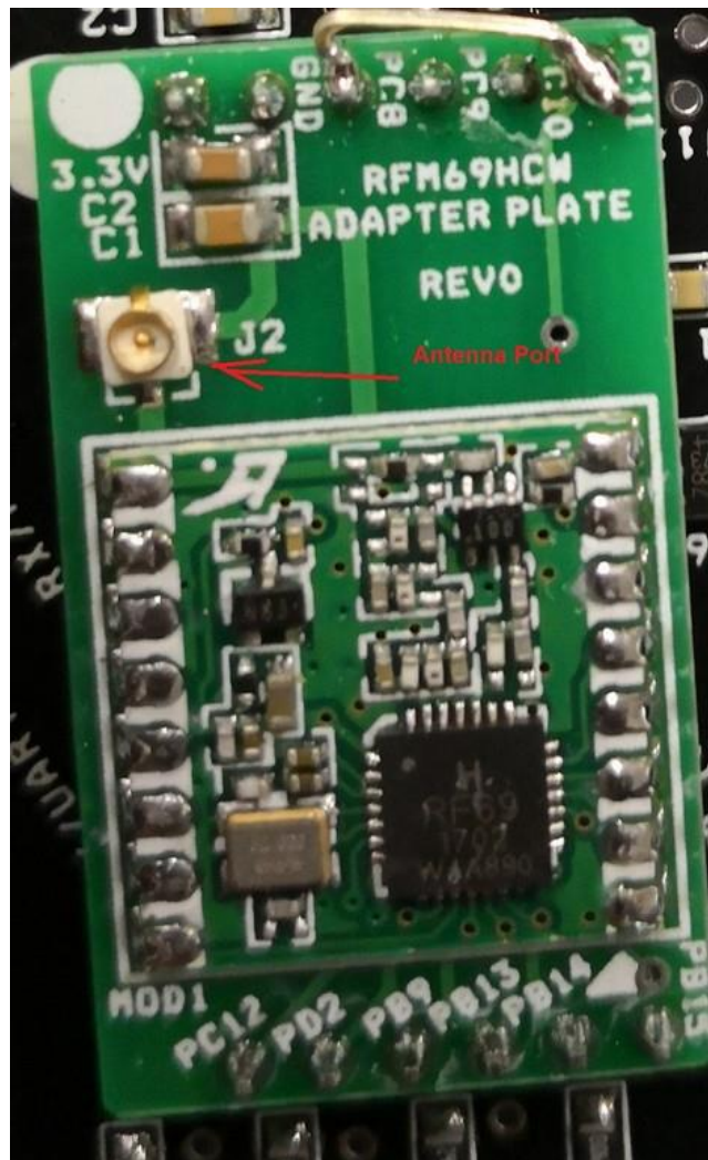
8.13 RFM69HCW Module PCB Components Side View
