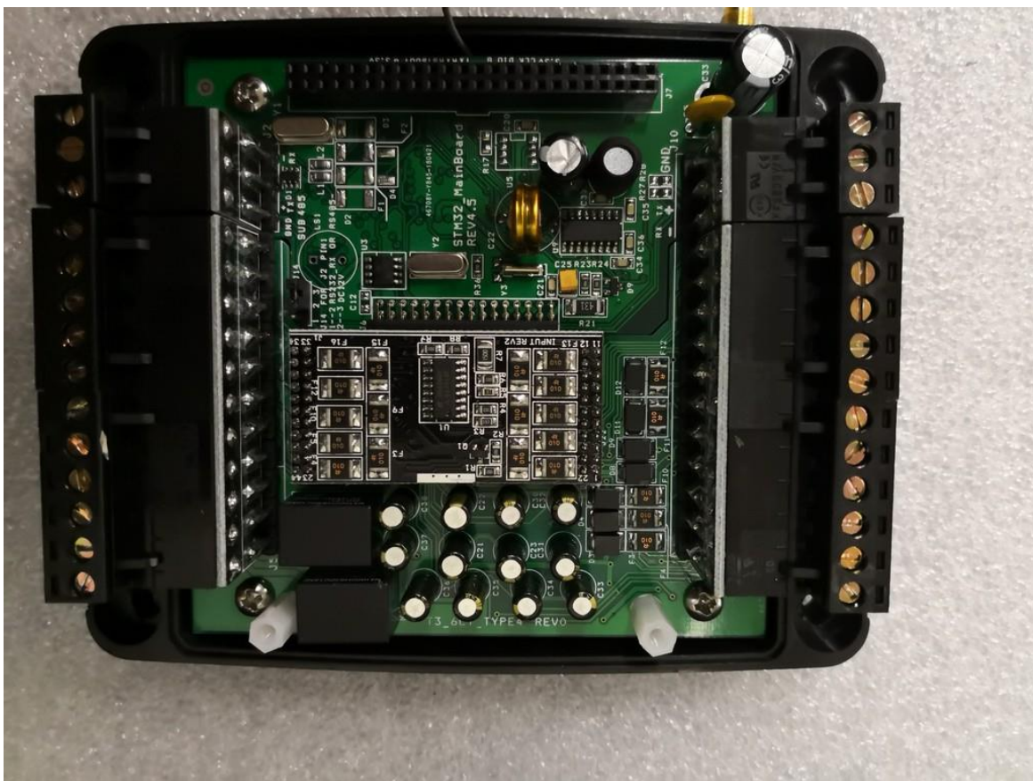
8.8 STEM32 Main Board Top Side View
