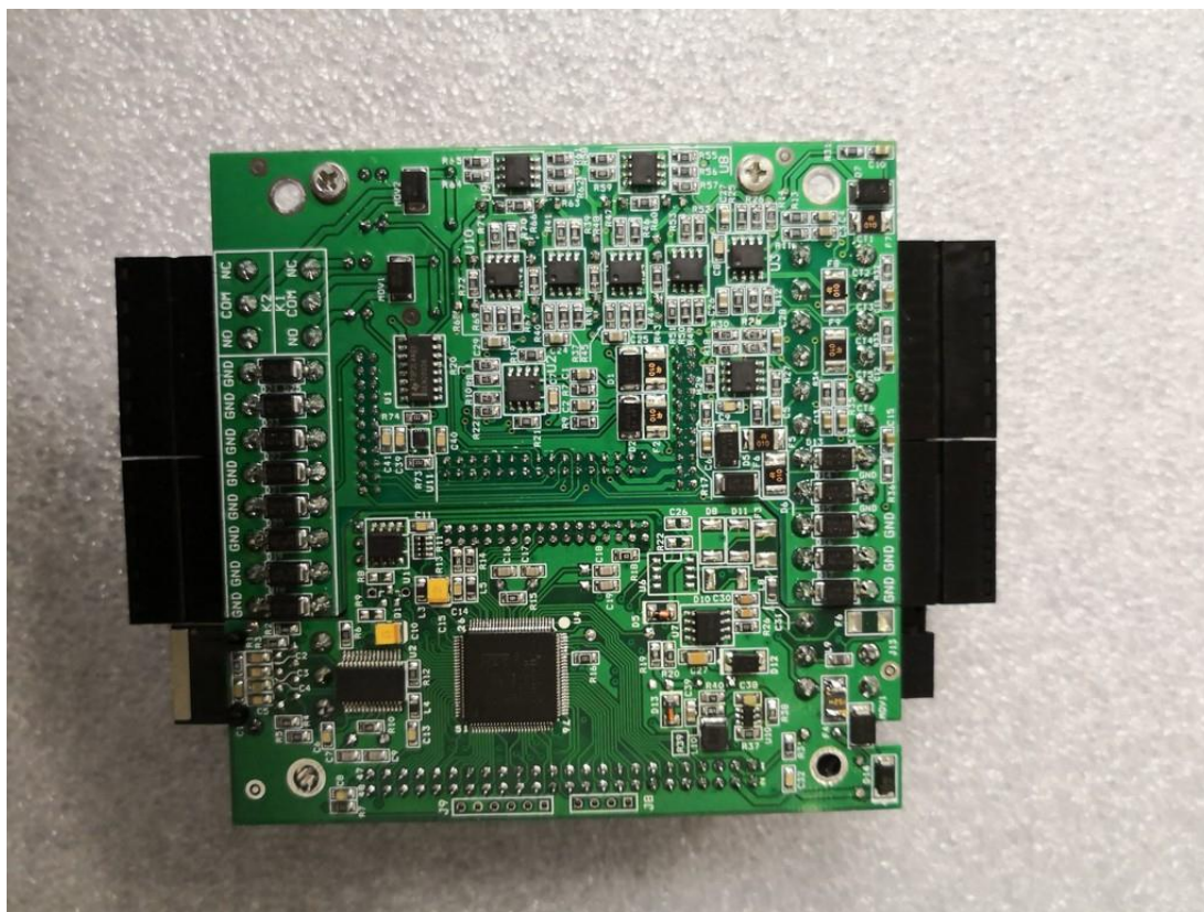
8.7 STEM32 Main Board Bottom Side View
