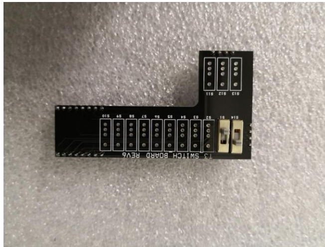
8.11 T3 Switch Board Front Side View
