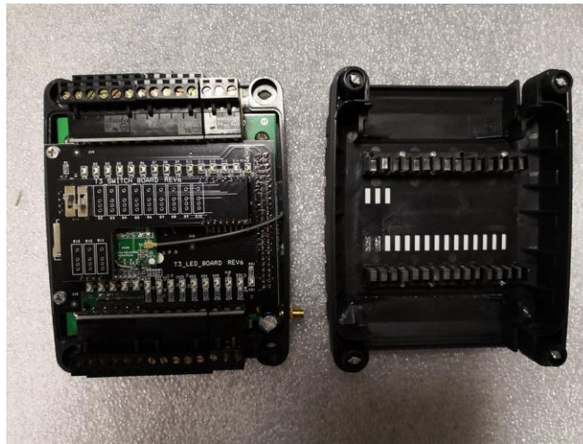
8.6 EUT Inside View
