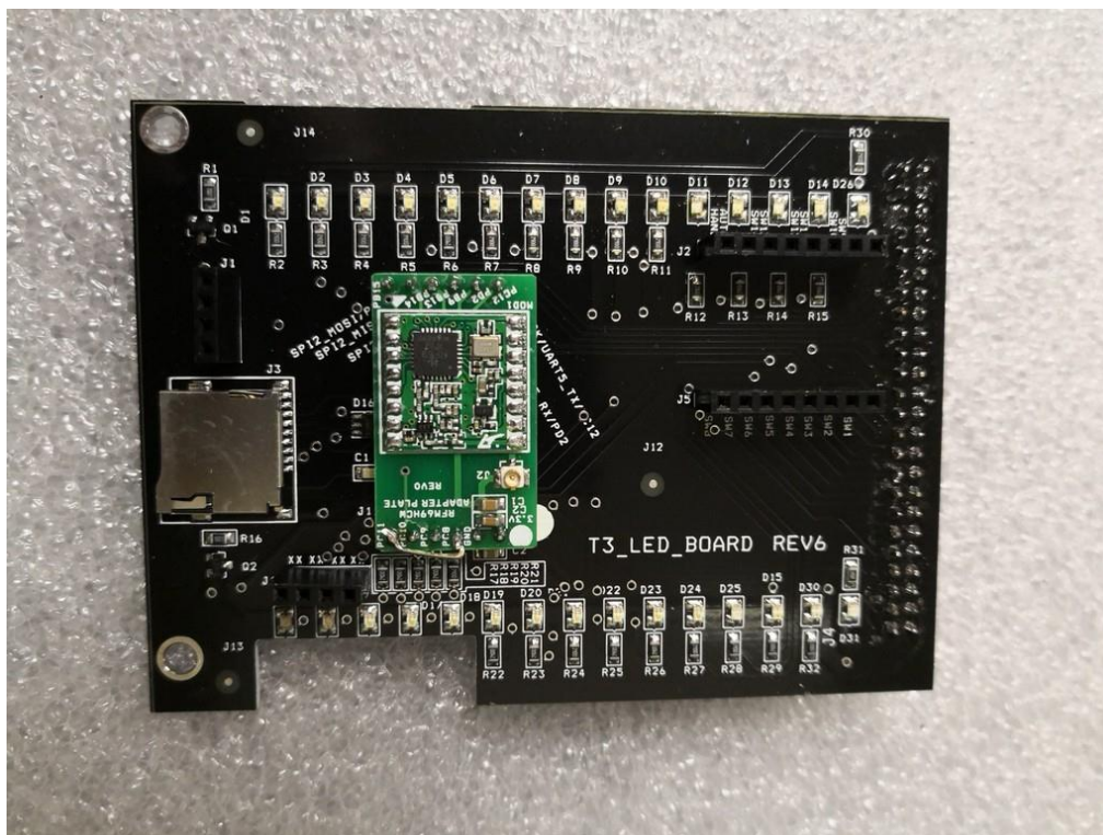
8.9 T3 LED Board Components Side View
