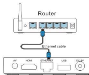
Ethernet cable connection
