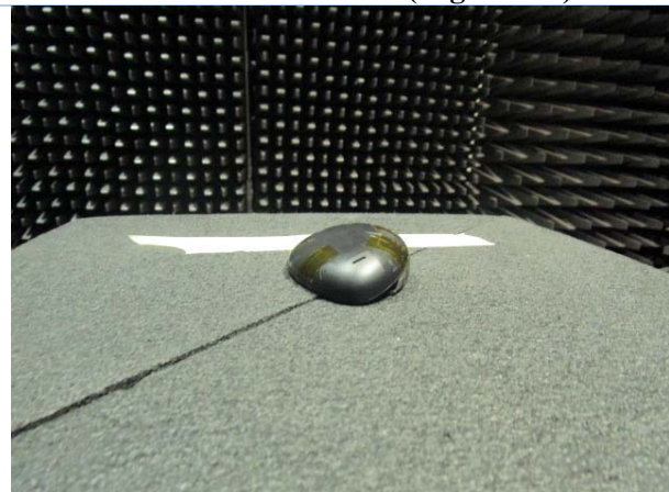
Radiated Emissions (Unit Flat) Chamber 5
