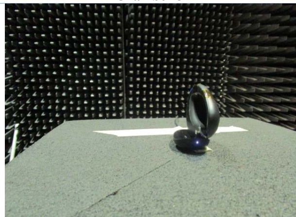
Radiated Emissions (Unit on Charger) Chamber 5
