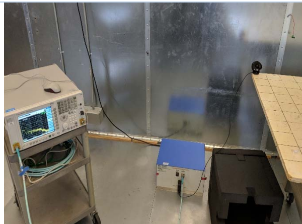
Conducted Emissions (Left Unit)
