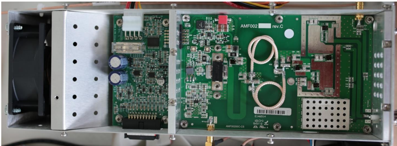
2.6 RF amplifier board
