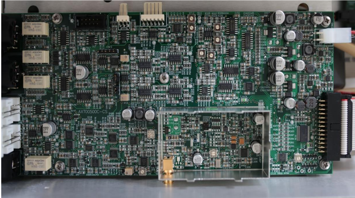
2.4 Interconnection board
