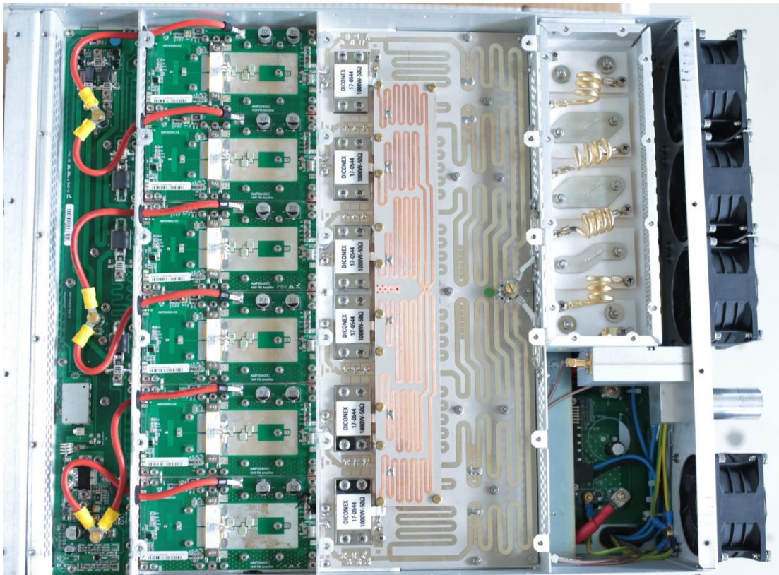
Bottom view
