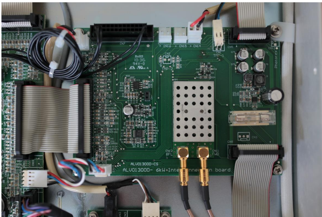
2.4 Interconnection board
