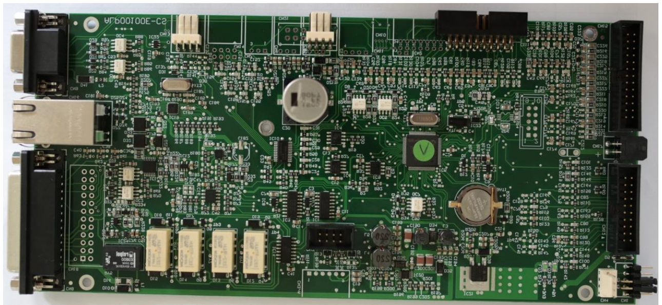
2.5 Logic board
