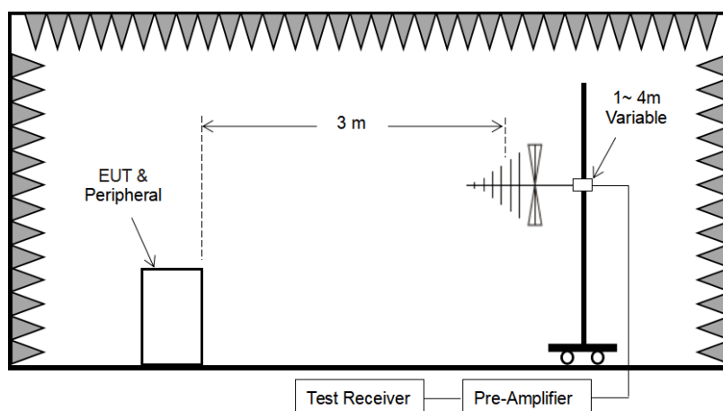
Figure 2. 30MHz to 1GHz
